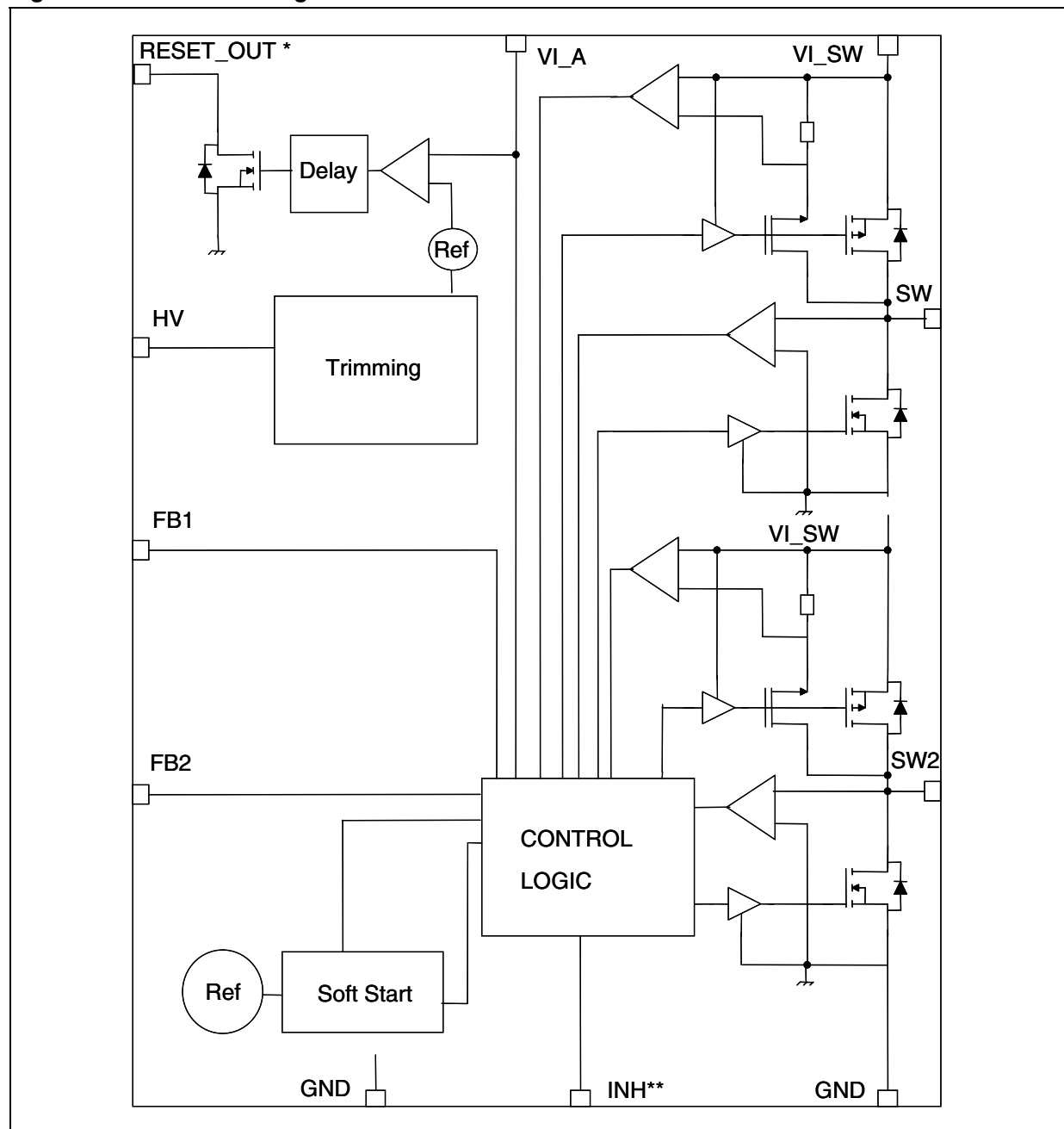
Figure 1. Schematic diagram
