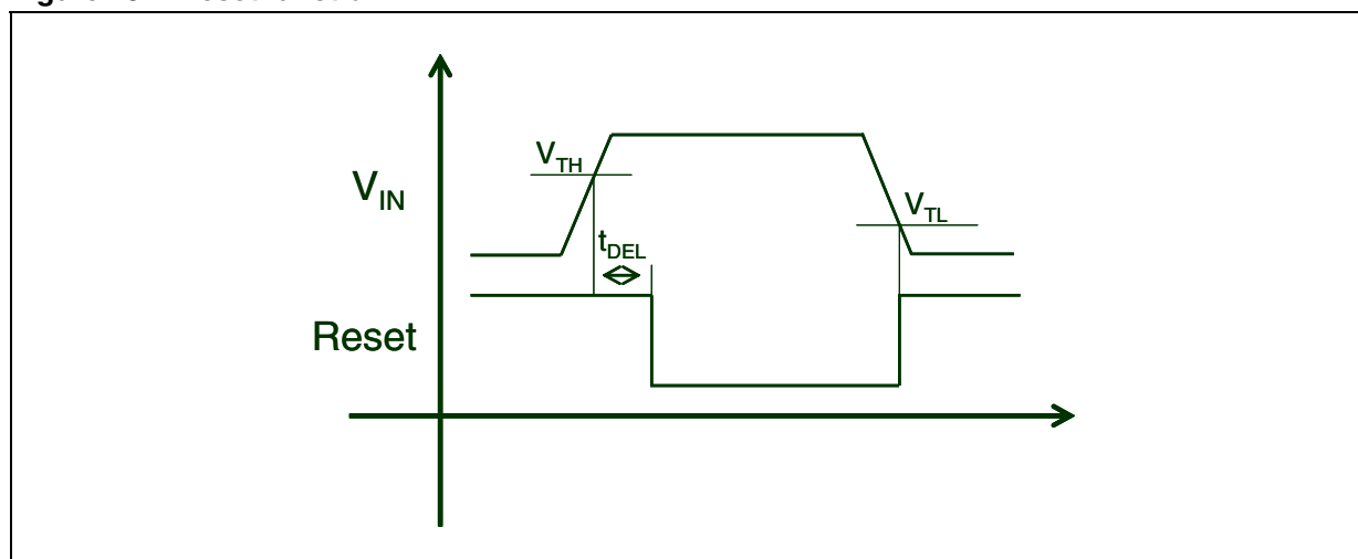
Figure 23. Reset function
