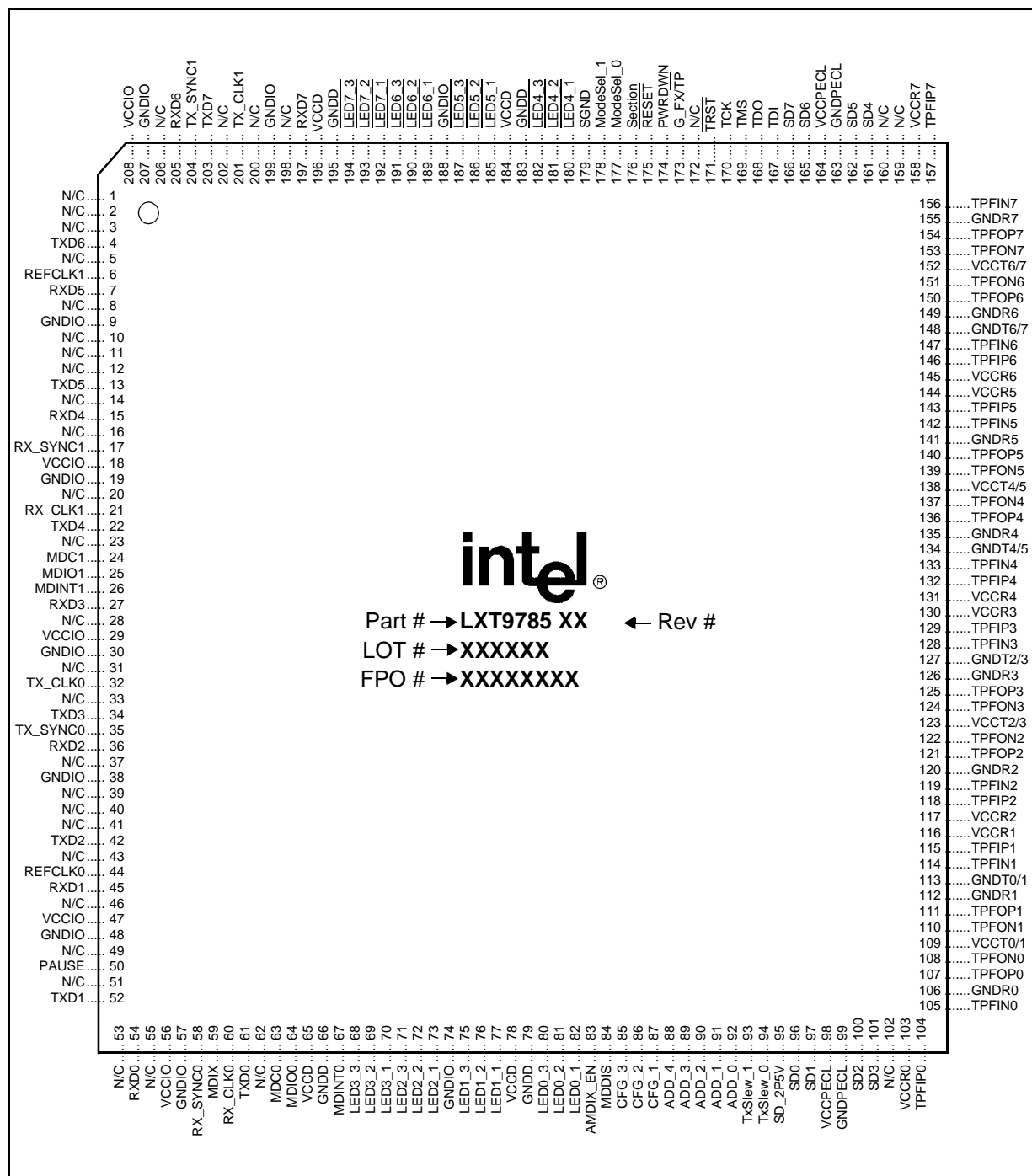
Figure 4. LXT9785 SS-SMII 208-Pin PQFP Assignments
