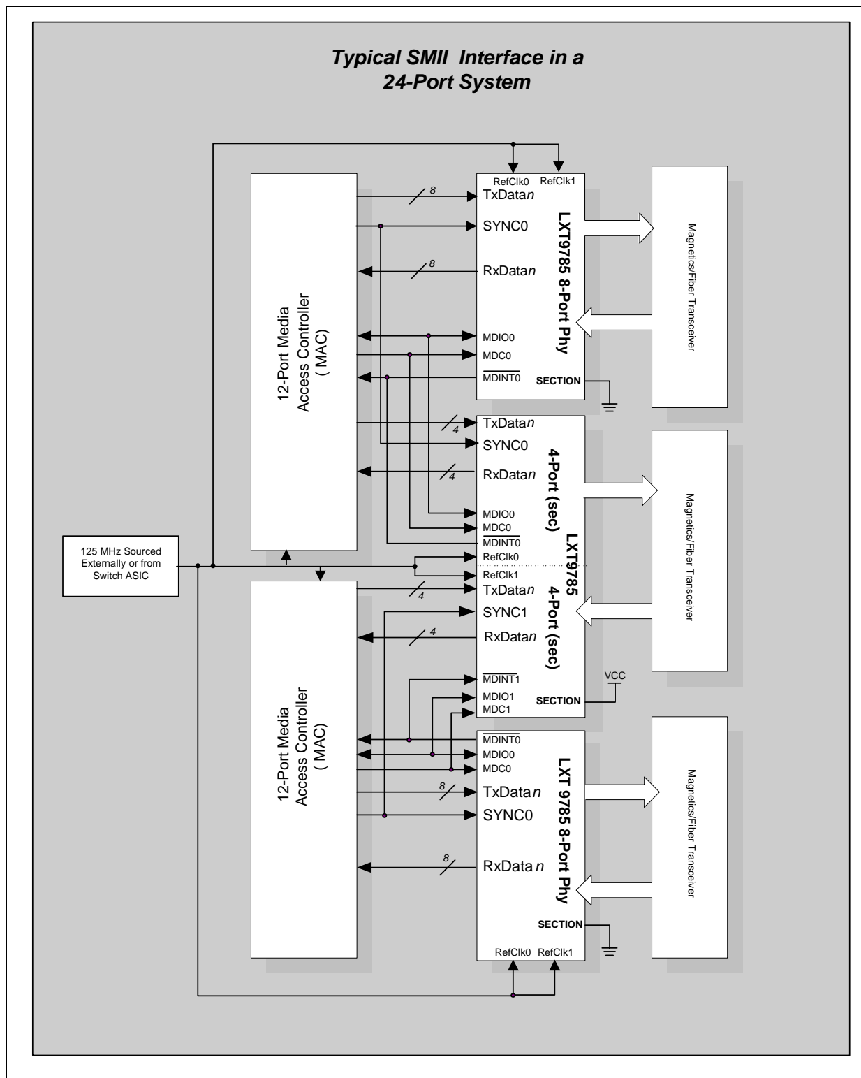
Figure 17. Typical SMII Quad Sectionalization Diagram
