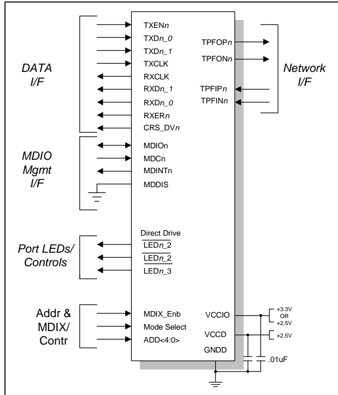
Figure 8. LXT9785 Interfaces
