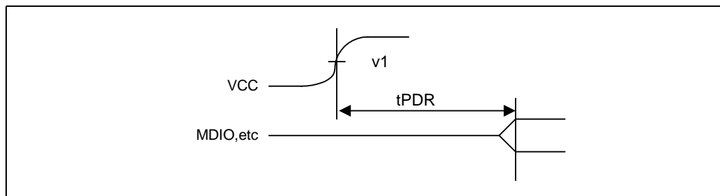
Figure 58. Power-Up Timing
