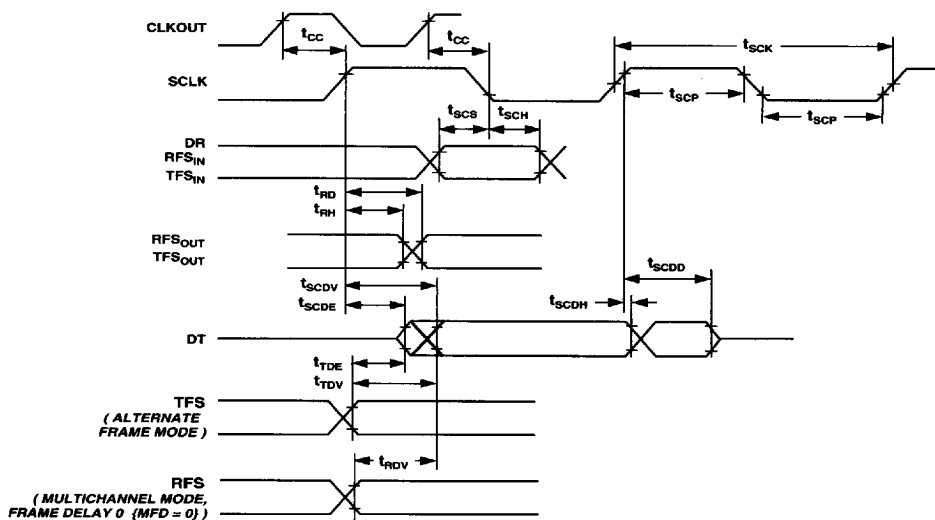
Figure 36. Serial Ports
