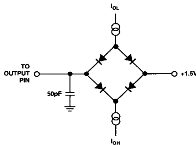
Figure 18. Equivalent Device Loading for AC Measurements (Except Output Enable/Disable)
