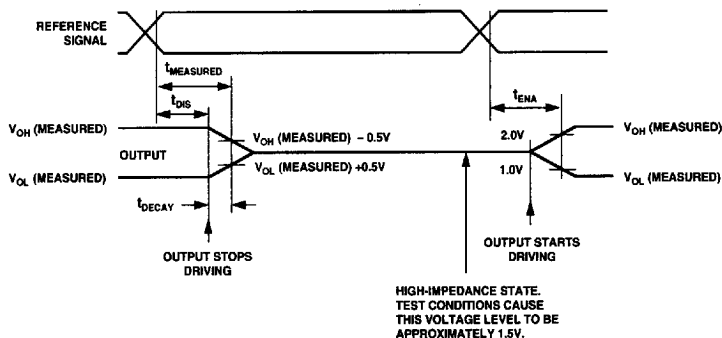
Figure 29. Output Enable/Disable
