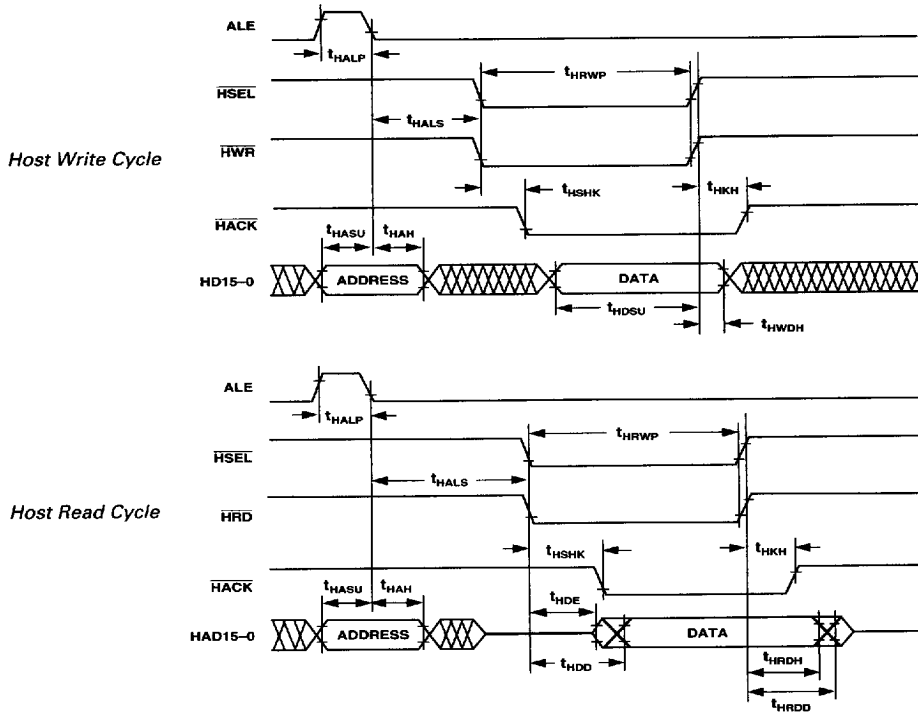
Figure 39. Host Interface Port (HMD1 = 1, HMD0 = 0)
