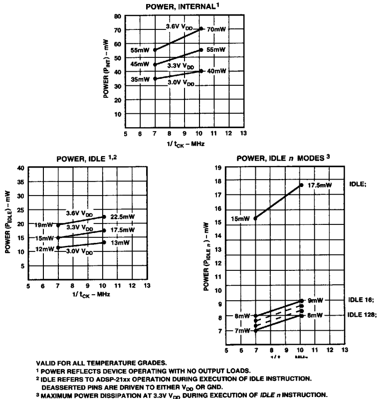
Figure 25. ADSP-2103 Power (Typical) vs. Frequency
