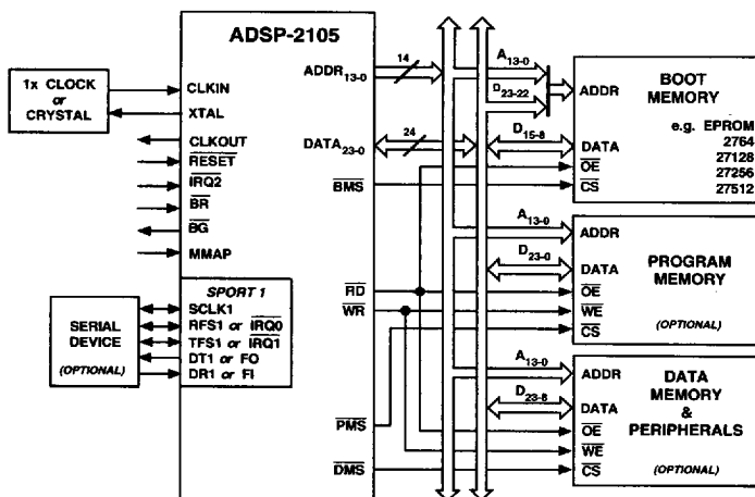
Figure 4. ADSP-2105 System
