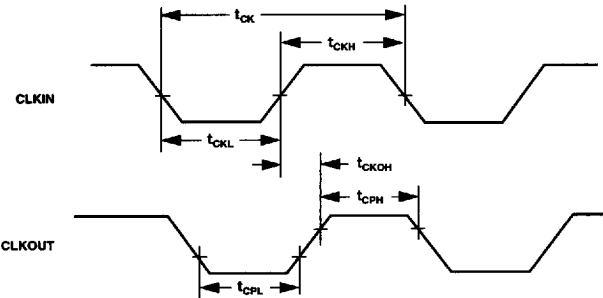
Figure 31. Clock Signals
