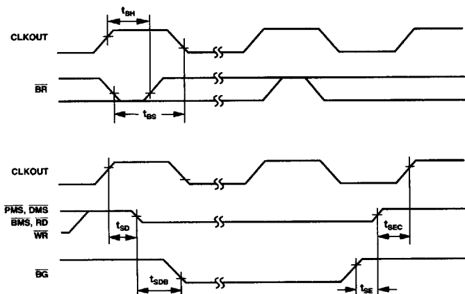
Figure 43. Bus Request/Grant
