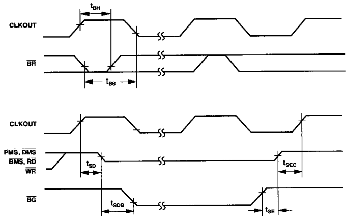
Figure 33. Bus Request/Grant
