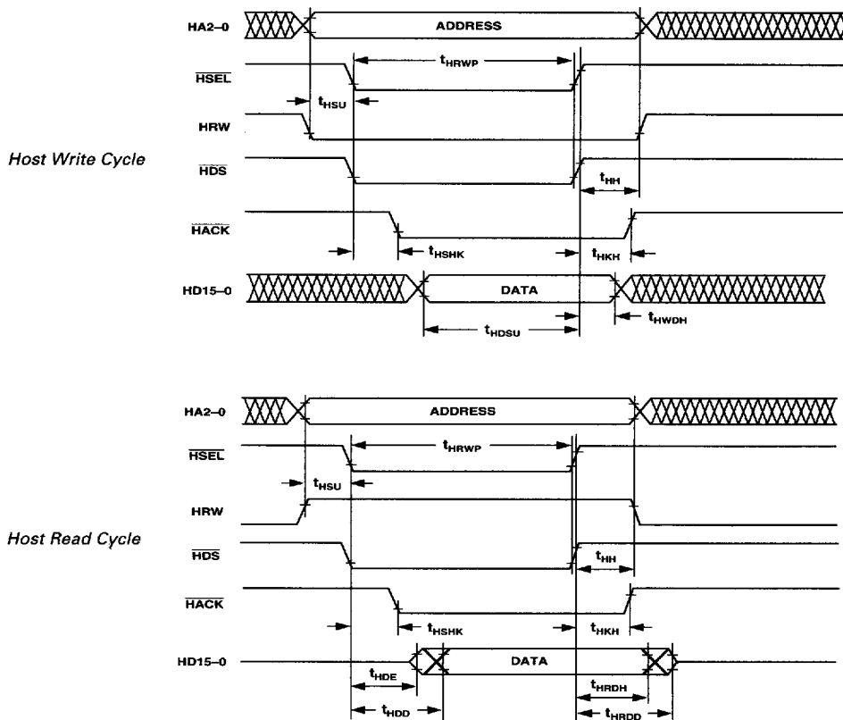
Figure 38. Host Interface Port (HMD1 = 0, HMD0 = 1)
