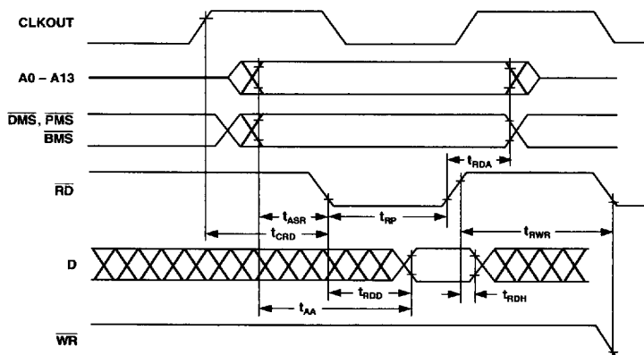
Figure 34. Memory Read
