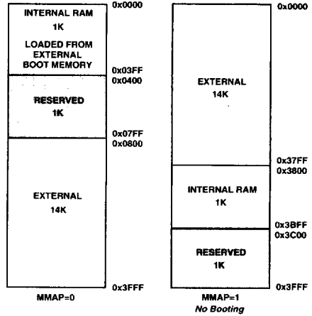
Figure 8. ADSP-2105/ADSP-2115 Program Memory Maps
