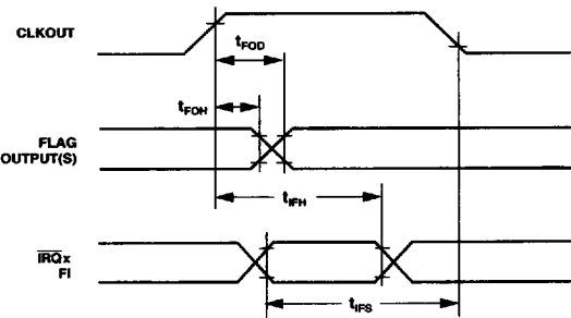
Figure 42. Interrupts & Flags
