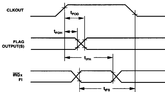
Figure 32. Interrupts &amp; Flags
