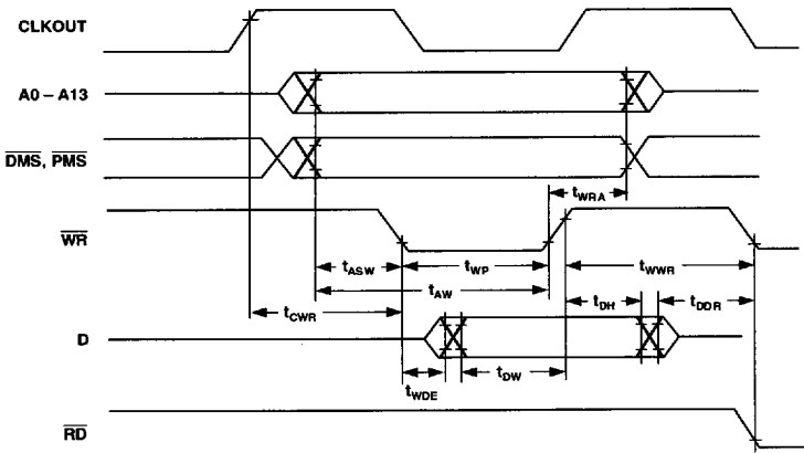
Figure 35. Memory Write
