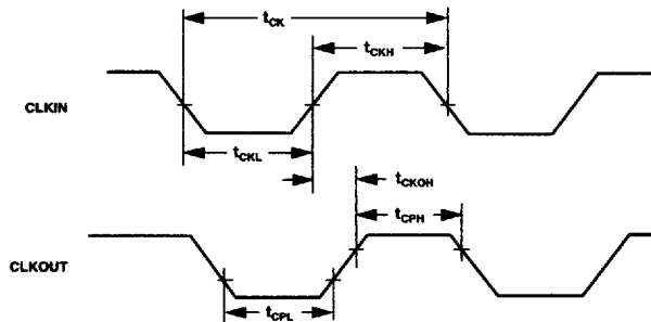
Figure 41. Clock Signals
