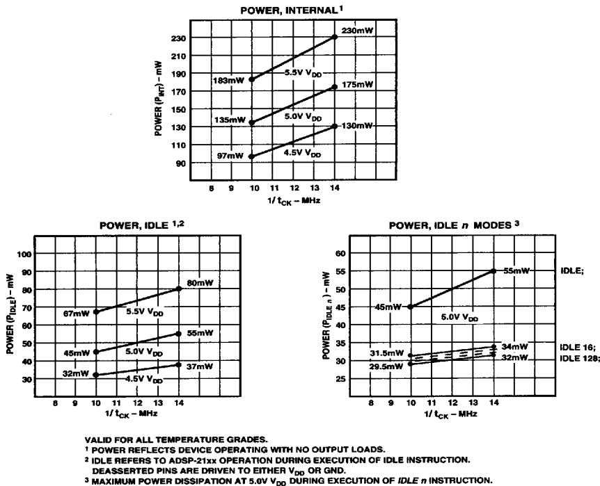
Figure 13. ADSP-2105 Power (Typical) vs. Frequency
