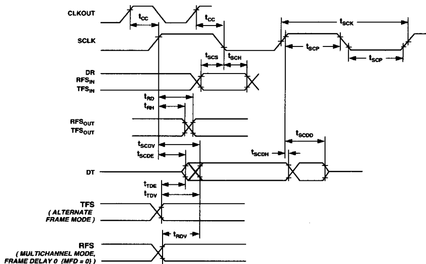
Figure 46. Serial Ports
