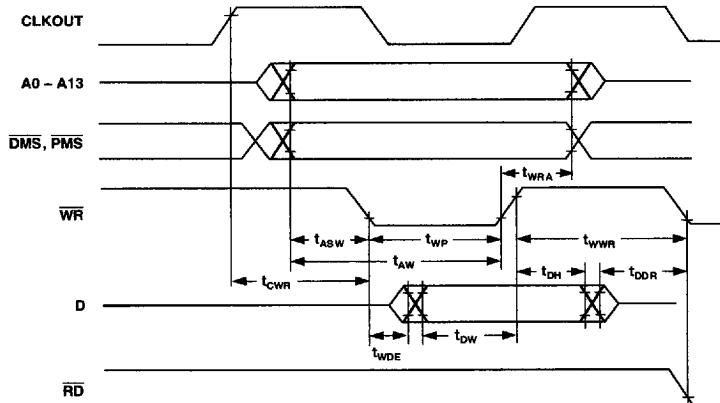
Figure 45. Memory Write
