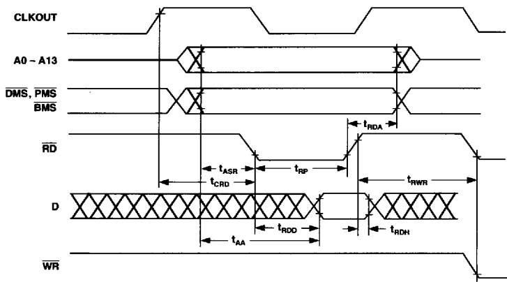
Figure 44. Memory Read
