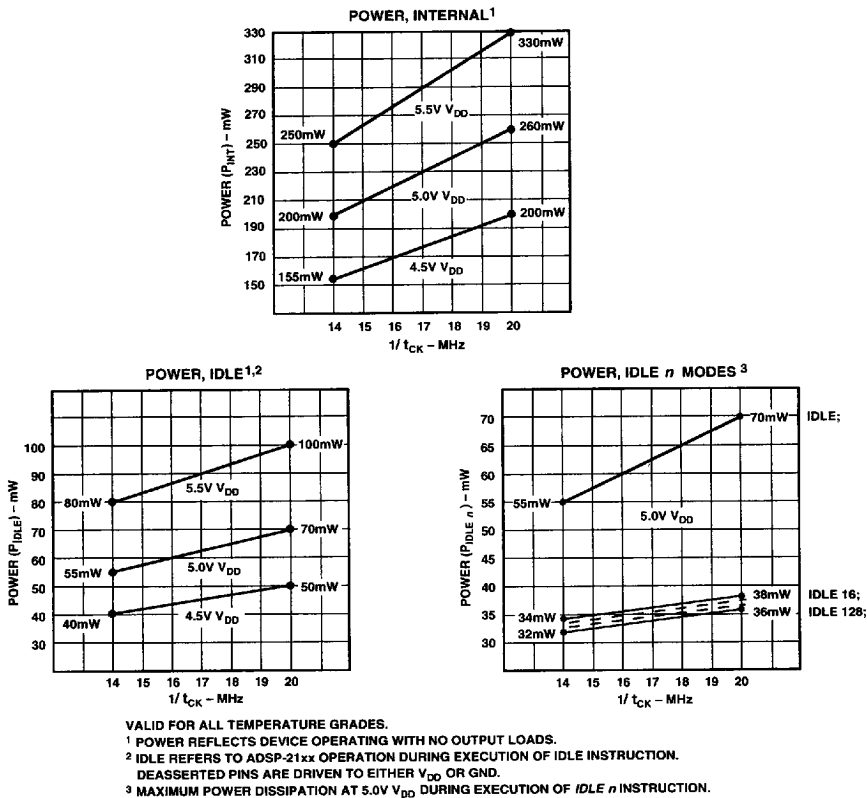
Figure 19. ADSP-2111 Power (Typical) vs. Frequency
