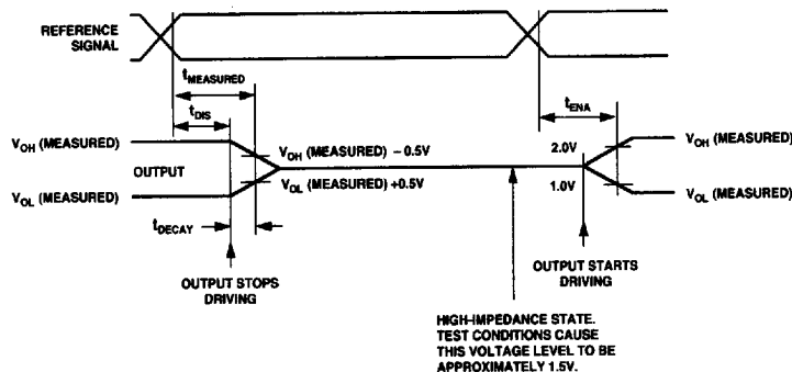
Figure 23. Output Enable/Disable
