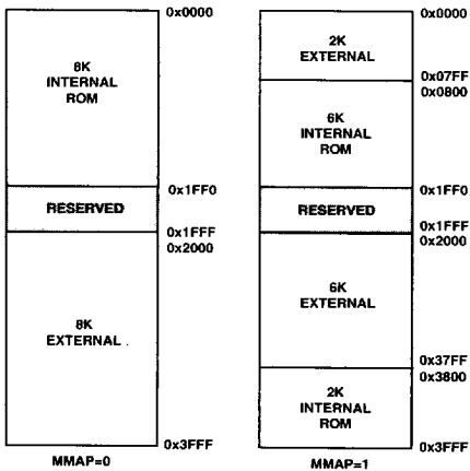
Figure 7. ADSP-2161/62 Program Memory Maps
