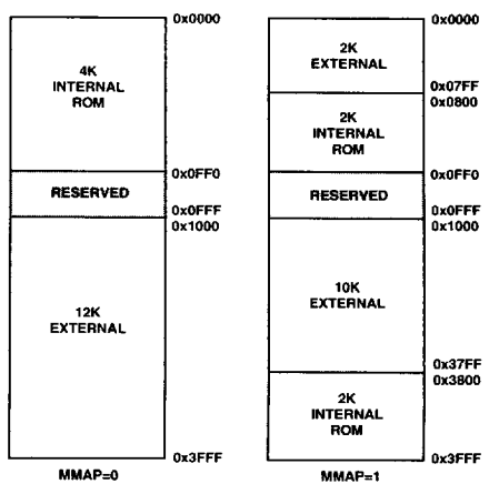
Figure 9. ADSP-2163/64 Program Memory Maps
