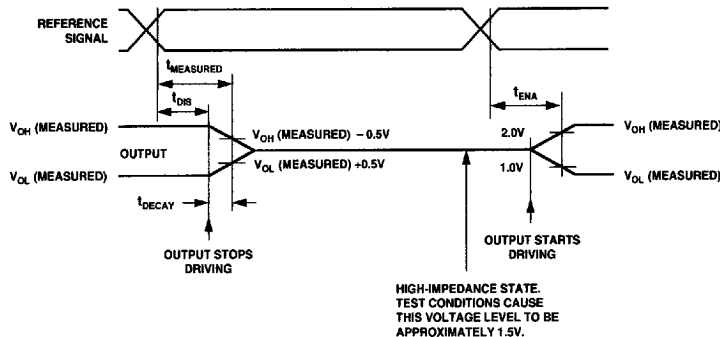
Figure 17. Output Enable/Disable
