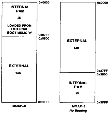
Figure 6. ADSP-2101/ADSP-2103/ADSP-2111 Program Memory Maps
