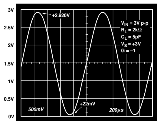
Figure 31. Output Swing, V_S = +3V
