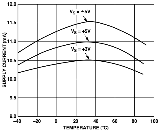
Figure 22. Supply Current vs. Temperature
