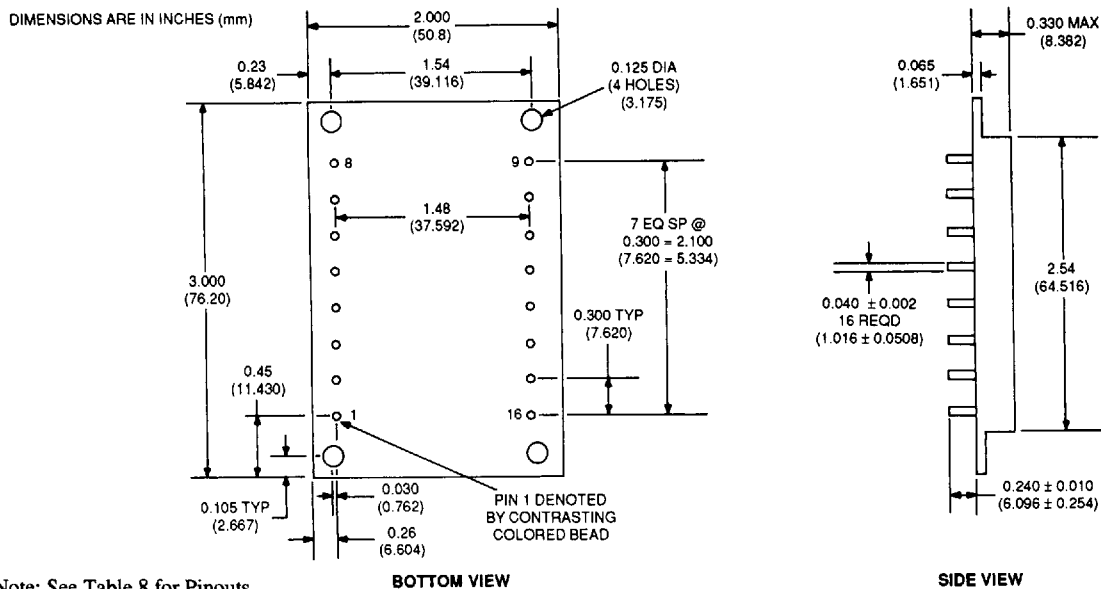
FIGURE 5. MECHANICAL OUTLINE FOR OPTIONAL 7-15 AMP DIP PACKAGING
