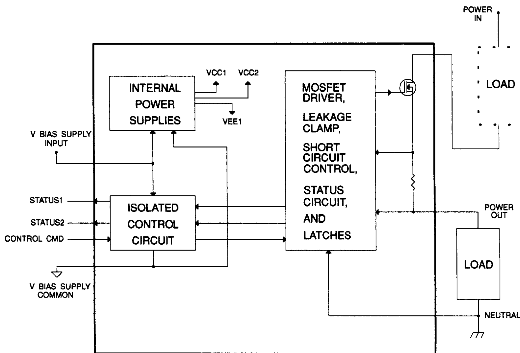
FIGURE 1. SSP-21116 BLOCK DIAGRAM
