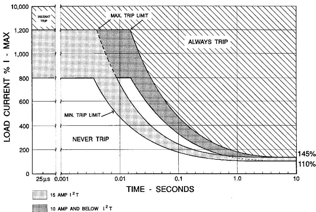
FIGURE 2. TRIP CHARACTERISTICS
