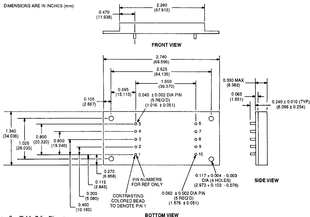
FIGURE 4. MECHANICAL OUTLINE FOR OPTIONAL 2-5 AMP PACKAGING
