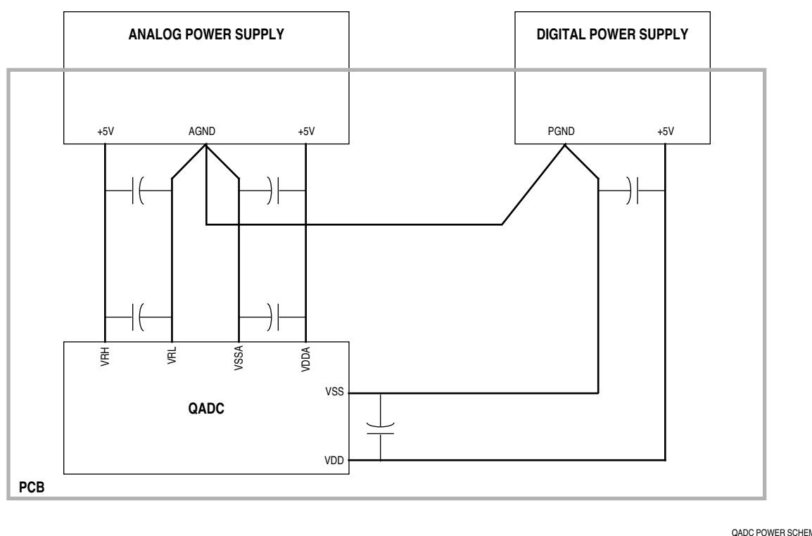
Figure 5-3 Star-Ground at the Point of Power Supply Origin
