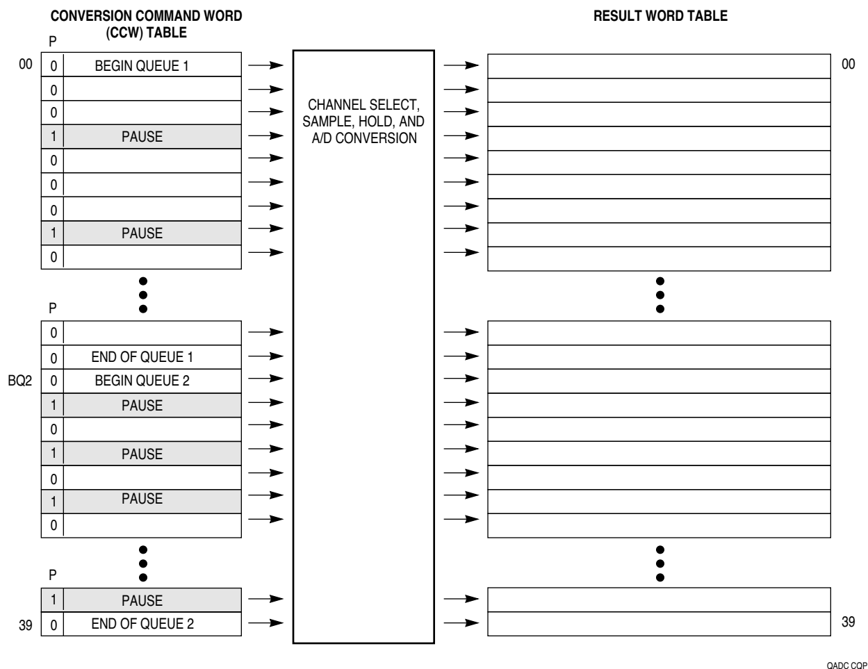
Figure 7-1 QADC Queue Operation With Pause
