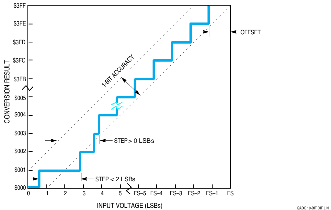
Figure C-5 Transfer Curve of a 10-Bit A/D Converter With Differential Linearity
