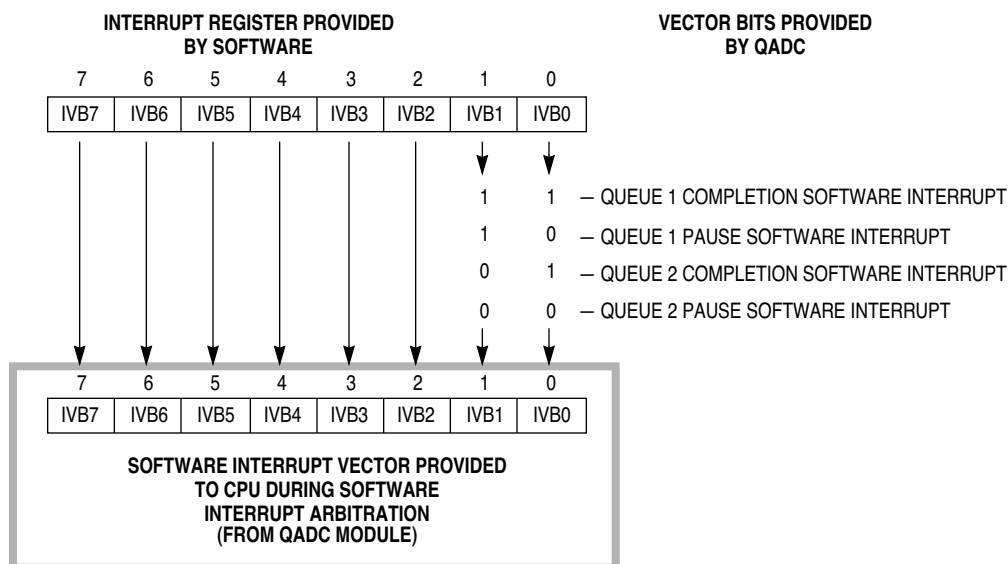
Figure 8-2 QADC Interrupt Vector Format
