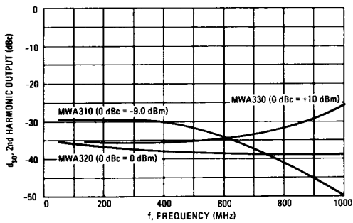
FIGURE 21 – SECOND HARMONIC OUTPUT versus FREQUENCY
