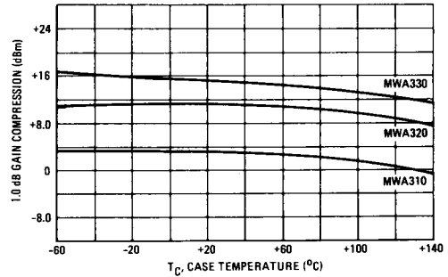
FIGURE 18 – 1.0 dB GAIN COMPRESSION versus CASE TEMPERATURE f = 1000 \text{ MHz}
