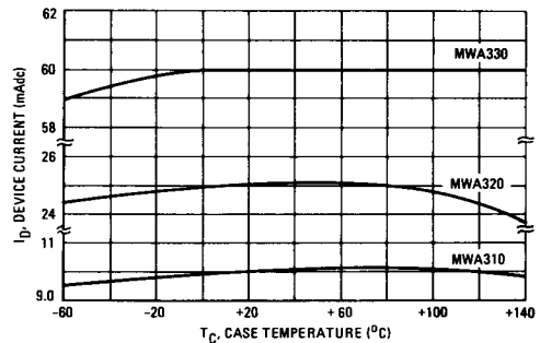
FIGURE 2 – DEVICE CURRENT versus CASE TEMPERATURE
