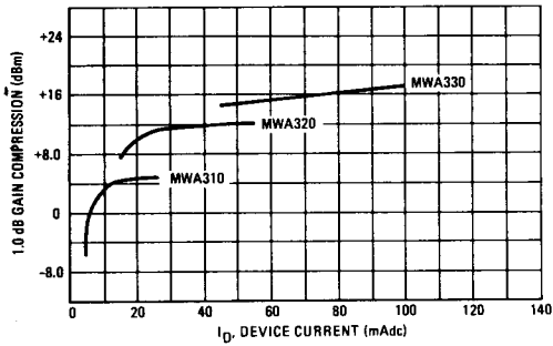
FIGURE 17 – 1.0 dB GAIN COMPRESSION versus DEVICE CURRENT f = 1000 \text{ MHz}
