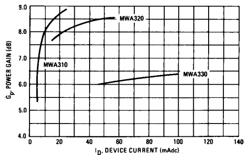
FIGURE 4 – POWER GAIN versus DEVICE CURRENT f = 1000 MHz
