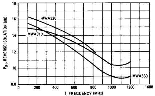
FIGURE 20 – REVERSE ISOLATION versus FREQUENCY
