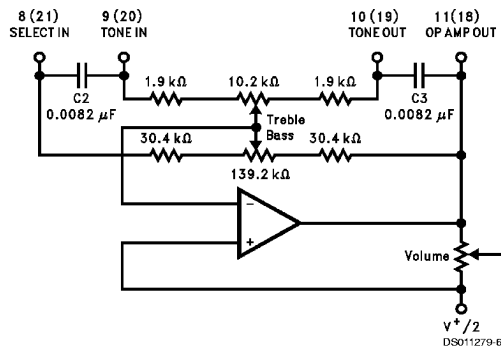
FIGURE 4. The Tone Control Amplifier
