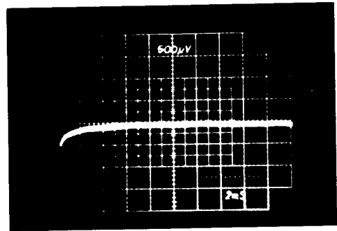
Hold Mode Dielectric Absorption Sag For 5 \mu sec Sample Period With Dielectric Absorption Compensation
