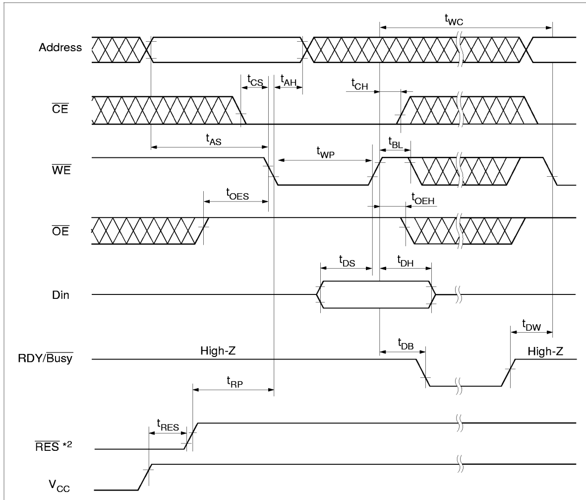
Byte Write Timing Waveform(1) ( \overline{\text{WE}} Controlled)
