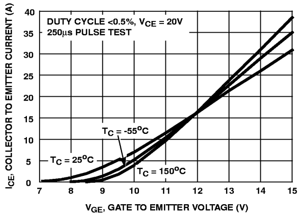
FIGURE 13. TRANSFER CHARACTERISTIC
