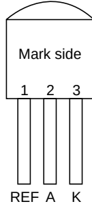
TO-92 (HA17L431P/AP)
