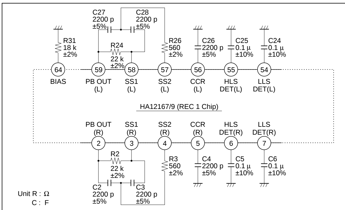
Figure 8 Tolerances of External Components
