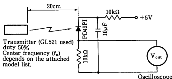
Fig. 1 Transmitter
