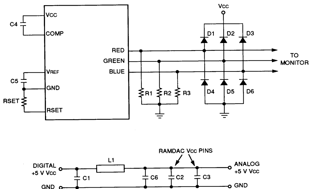
Figure 6. Typical Connection Diagram for Internal Voltage Reference
