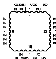
LCC/PLCC
