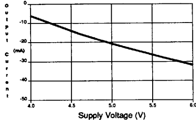
OUTPUT SOURCE CURRENT vs. SUPPLY VOLTAGE (VOH = 2.4V)
