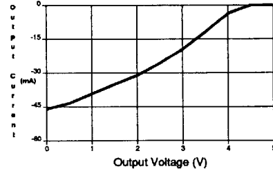
OUTPUT SOURCE CURRENT vs. OUTPUT VOLTAGE (TA = 25°C, VCC = 5V)
