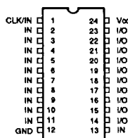
DIP/SOIC
