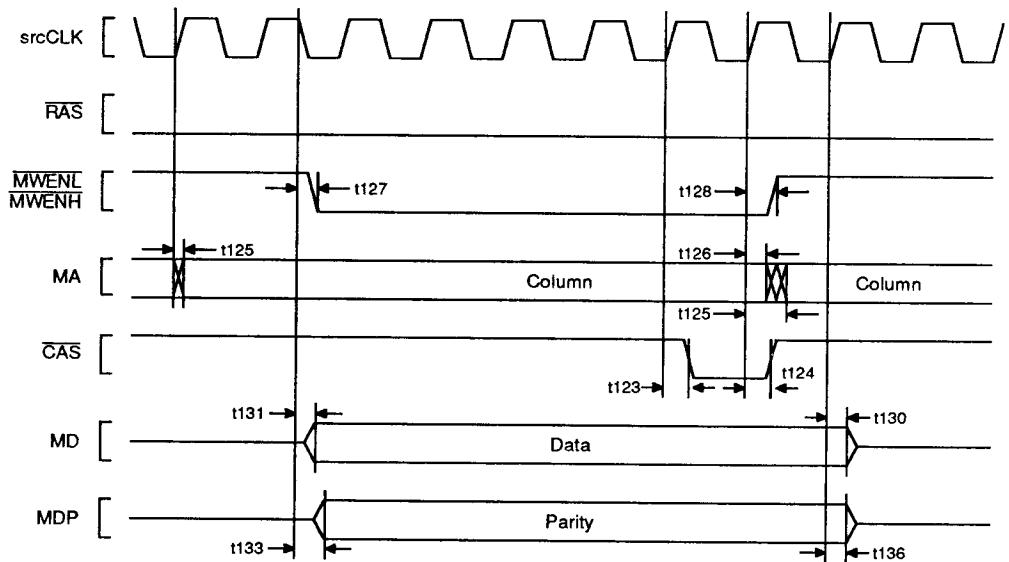
Figure 38. M Bus: Page Mode, Page—Hit \overline{\text{RAS}} Active/Write/1WS
