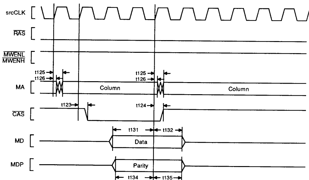
Figure 39. M Bus: Page Mode, Page—Hit \overline{\text{RAS}} Active/0WS/Read
