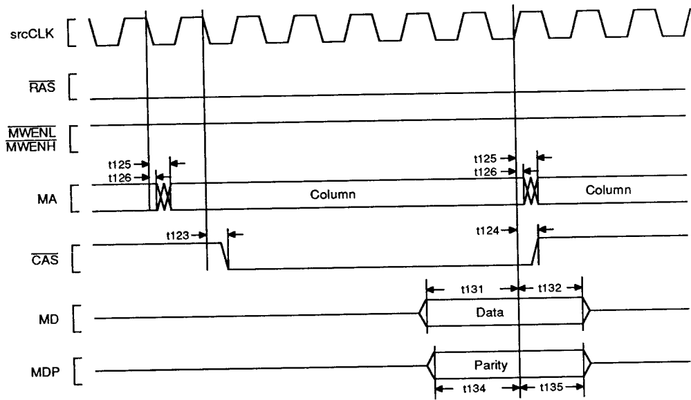
Figure 40. M Bus: Page Mode, Page—Hit RAS Active/1WS/Read
