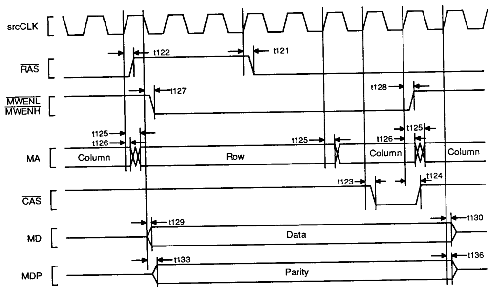
Figure 40. M Bus: Page Mode, Page—Hit RAS Active/1WS/Read
