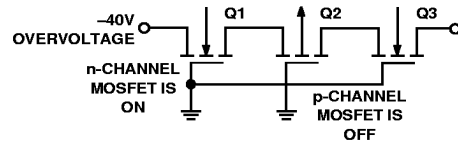
Figure 15. -40 V Overvoltage with Power OFF
