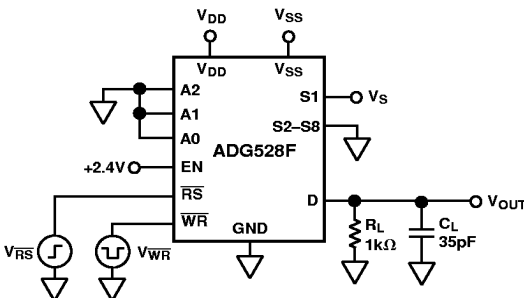
Test Circuit 10. Write Turn-On Time, t_{ON} (\overline{WR})
