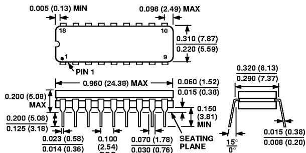
18-Lead Cerdip (Q-18)
