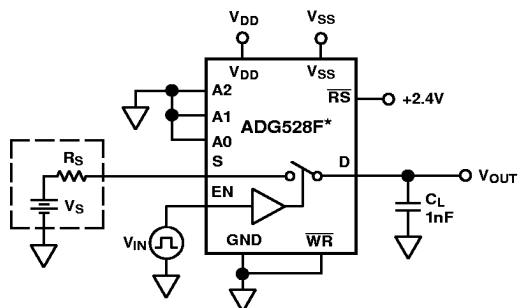
Test Circuit 11. Reset Turn-Off Time, t_{OFF}(\overline{RS})
