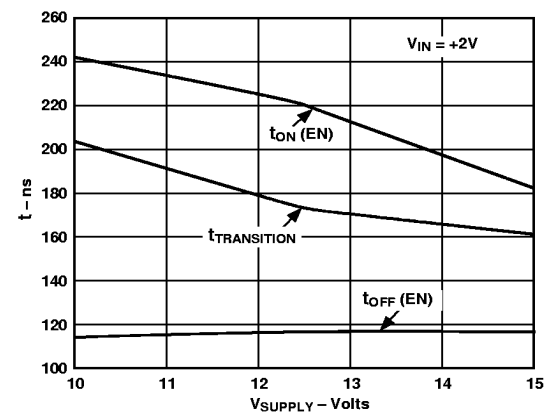
Figure 10. Switching Time vs. Power Supply
