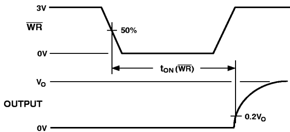
Test Circuit 10. Write Turn-On Time, t_{ON} (\overline{WR})
