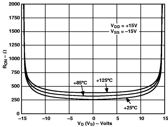
Figure 6. On Resistance as a Function of V_D ( V_S ) for Different Temperatures
