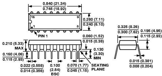
16-Lead Plastic (N-16)
