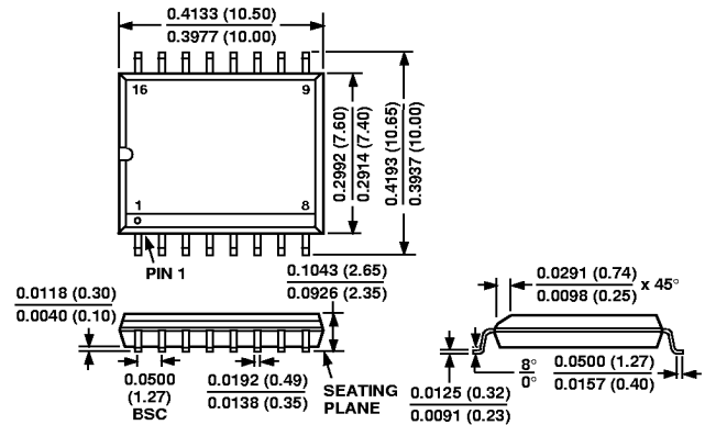
16-Lead SOIC (R-16W) (Wide Body)
