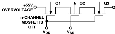
Figure 12. +55 V Overvoltage Input to the ON Channel
