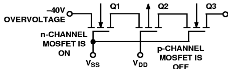
Figure 13. -40 V Overvoltage on an OFF Channel with Multiplexer Power ON
