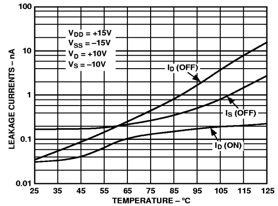
Figure 9. Leakage Currents as a Function of Temperature
