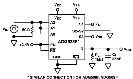
Test Circuit 7. Switching Time of Multiplexer, t_{TRANSITION}
