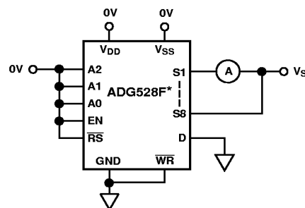
Test Circuit 5. Input Leakage Current (with Overtolerance)
