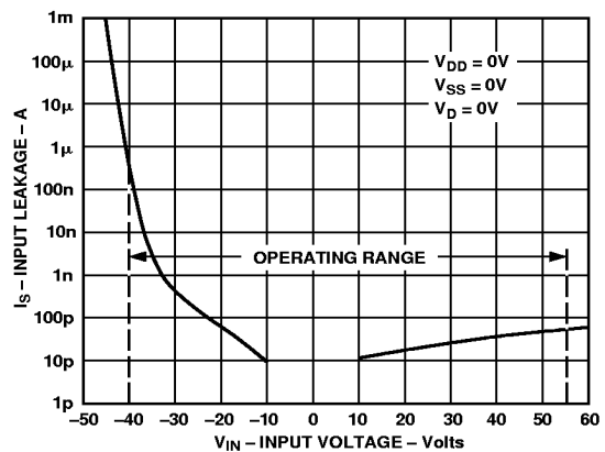
Figure 4. Input Leakage Current as a Function of V_S (Power Supplies OFF) During Overvoltage Conditions
