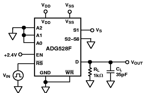
Test Circuit 11. Reset Turn-Off Time, t_{OFF}(\overline{RS})
