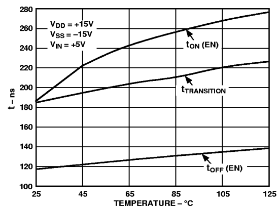
Figure 11. Switching Time vs. Temperature
