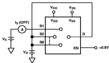
Test Circuit 2. I_S (OFF)
