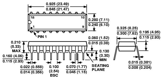
18-Lead Plastic (N-18)
