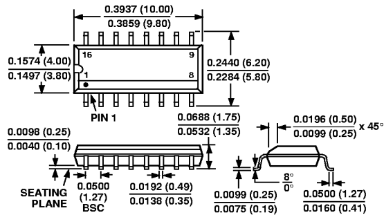
16-Lead SOIC (R-16N) (Narrow Body)
