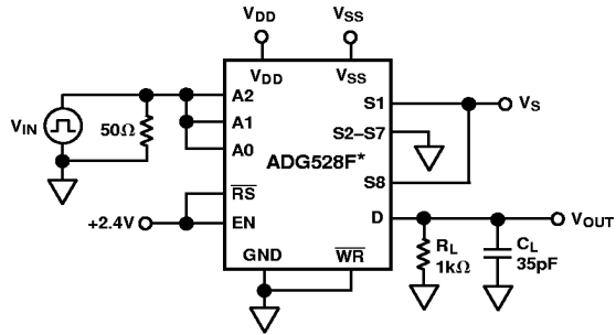
Test Circuit 8. Break-Before-Make Delay, t_{OPEN}
