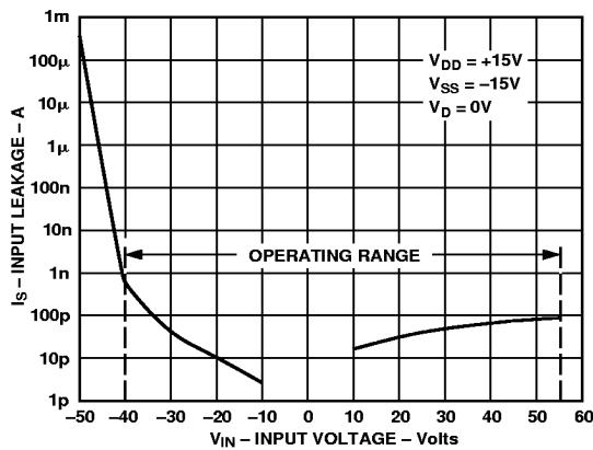
Figure 7. Input Leakage Current as a Function of V_S (Power Supplies ON) During Overvoltage Conditions
