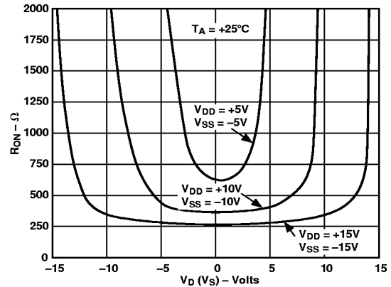
Figure 3. On Resistance as a Function of V_D ( V_S )
