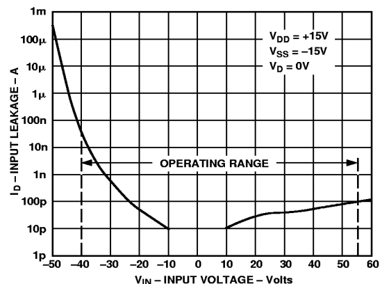
Figure 5. Output Leakage Current as a Function of V_S (Power Supplies ON) During Overvoltage Conditions
