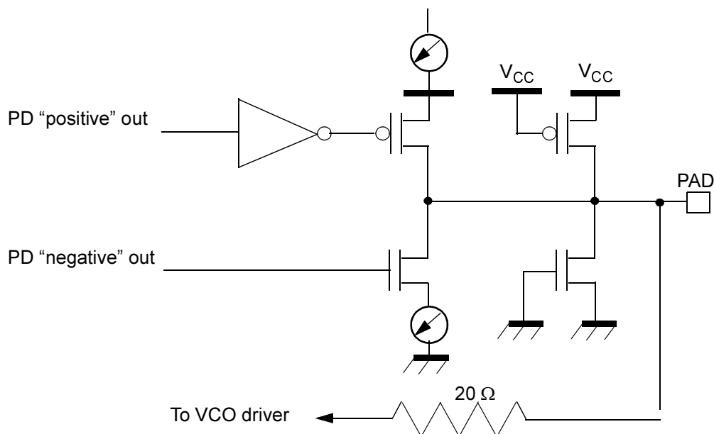
Figure 26 Loop Filter Pin Configuration
