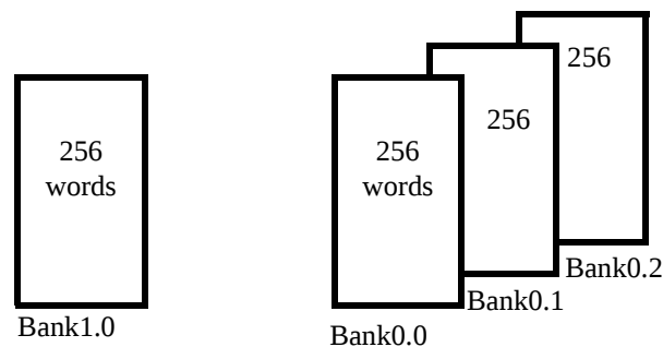
Figure 7 RAM Allocation
