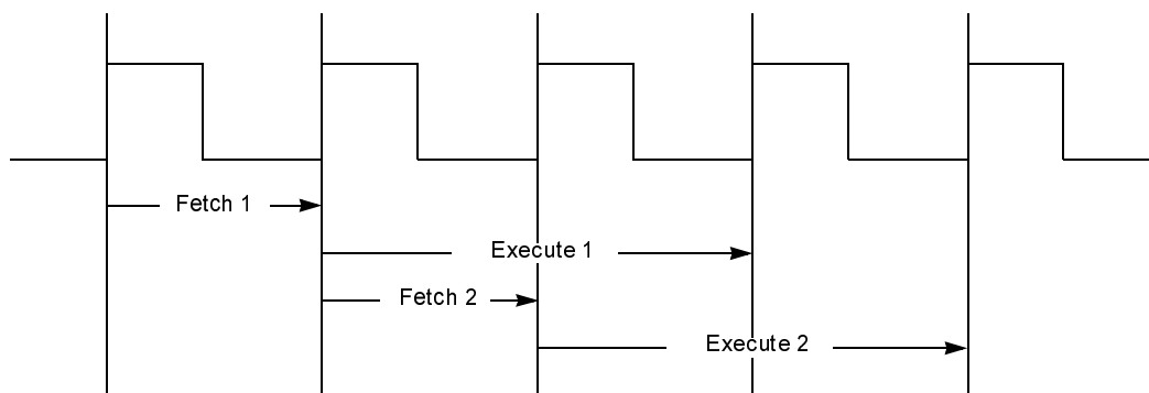
Figure 27 Pipeline Execution
