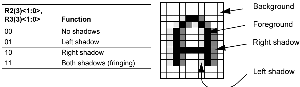
Figure 22 Table Settings
