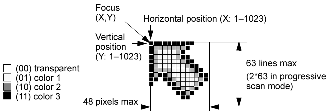
Figure 23 Cursor
