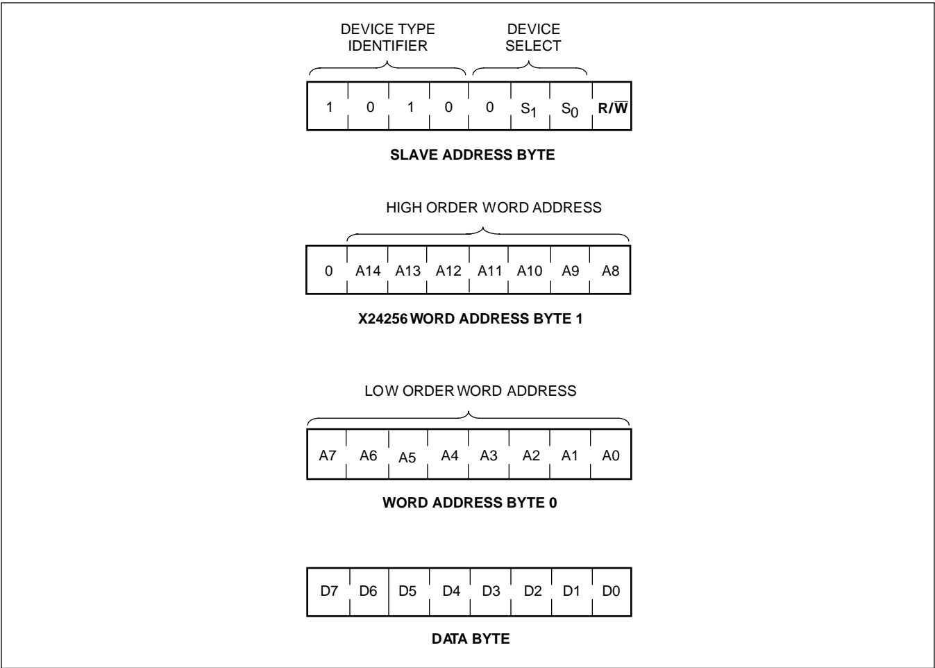
Figure 4. Device Addressing
