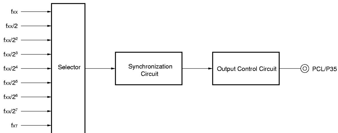
Figure 5-6. Clock Output Control Circuit Block Diagram
