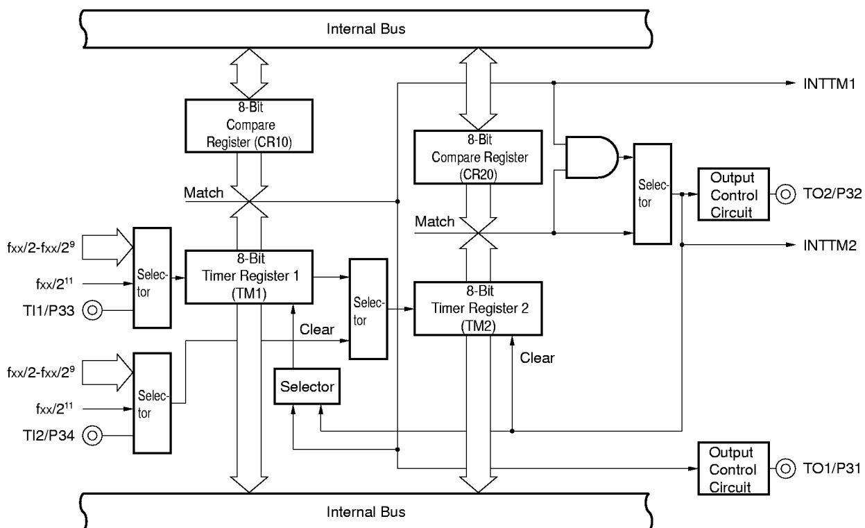
Figure 5-3. 8-Bit Timer/Event Counter Block Diagram
