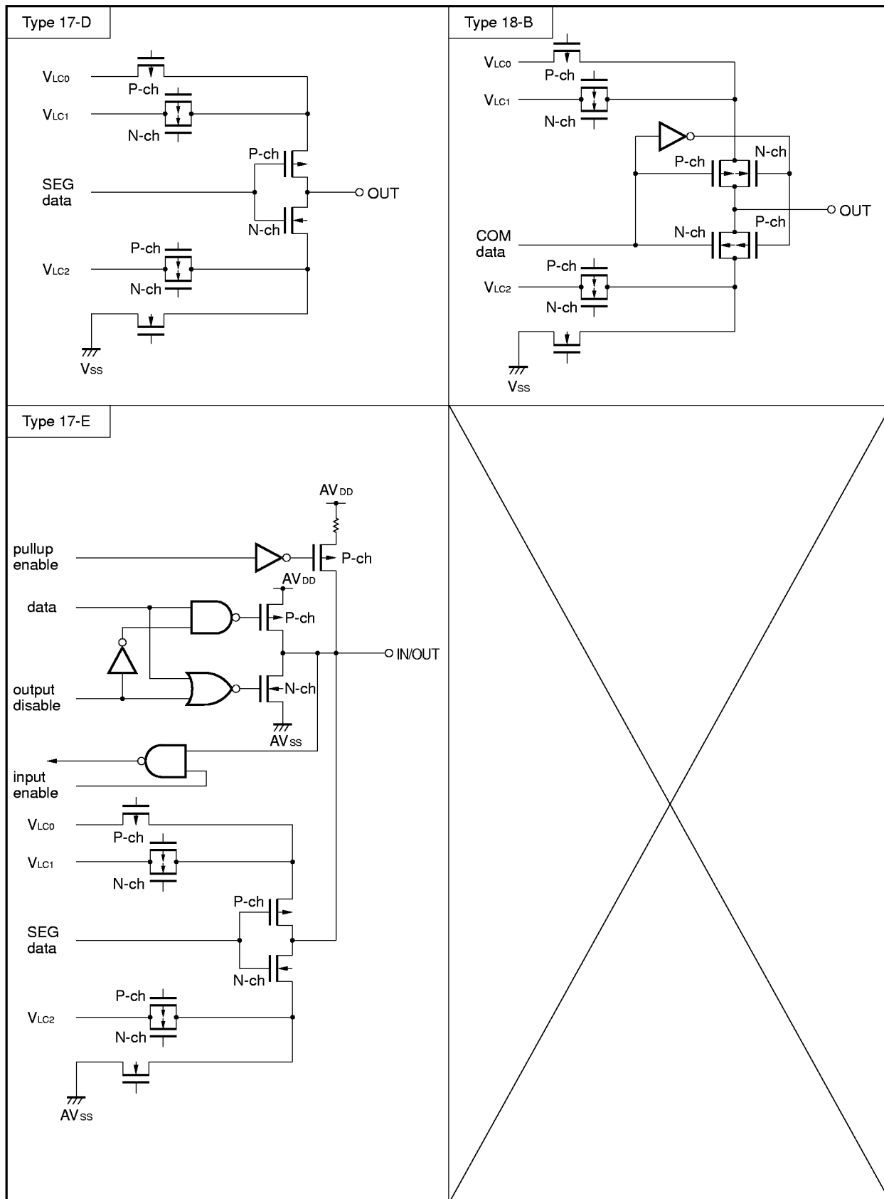
Figure 3-1. Pin Input/Output Circuits (2/2)
