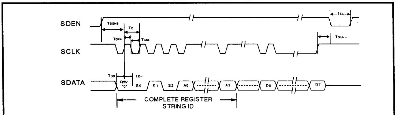
FIGURE 7: Serial Interface Timing
