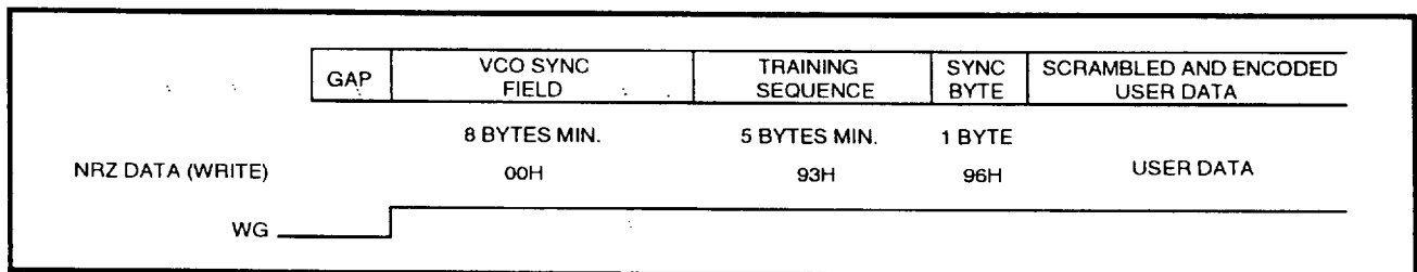
FIGURE 8: Hard Sector Write Sequence
