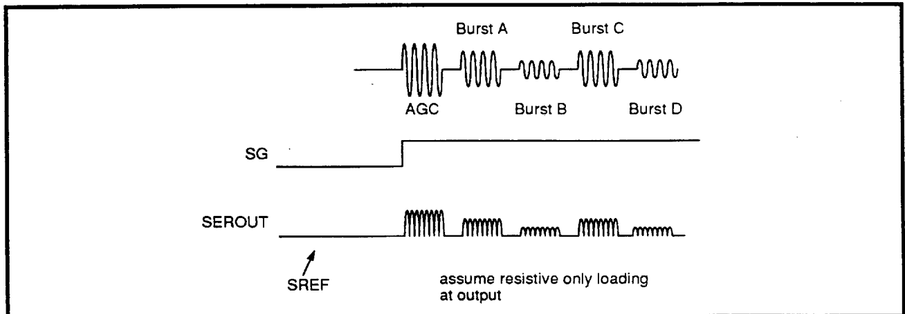
FIGURE 5: Servo Function Diagram
