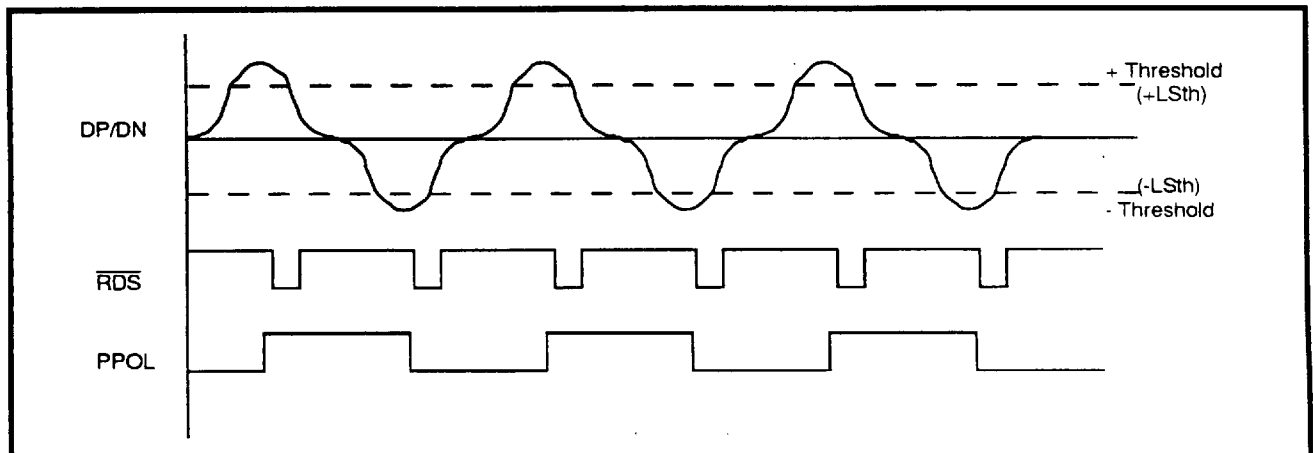
FIGURE 6: \overline{RDS} and PPOL vs. DP/DN Relationship
