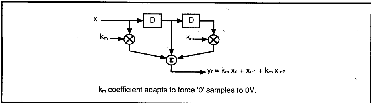
FIGURE 2: Block Diagram of 3-Tap Adaptive Equalizer
