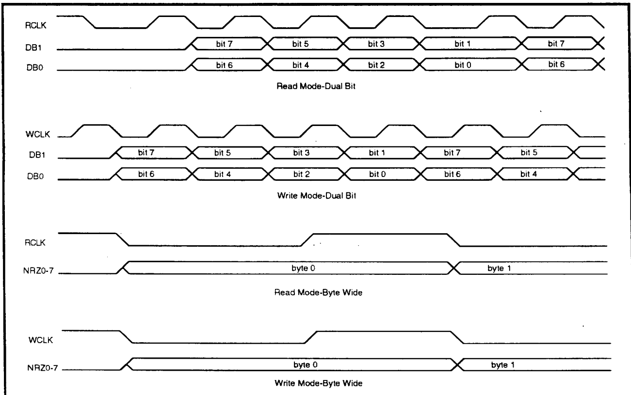
FIGURE 4: RCLK, WCLK vs. NRZ Data
