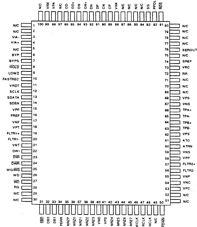
100-Lead QFP
