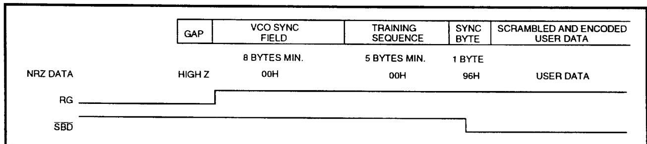
FIGURE 9: Hard Sector Read Sequence
