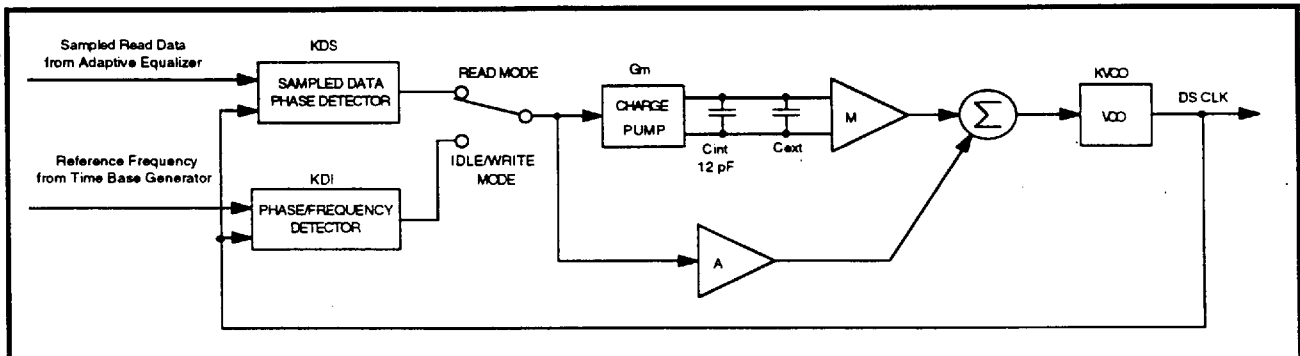
FIGURE 3: Data Synchronizer Phase Locked Loop
