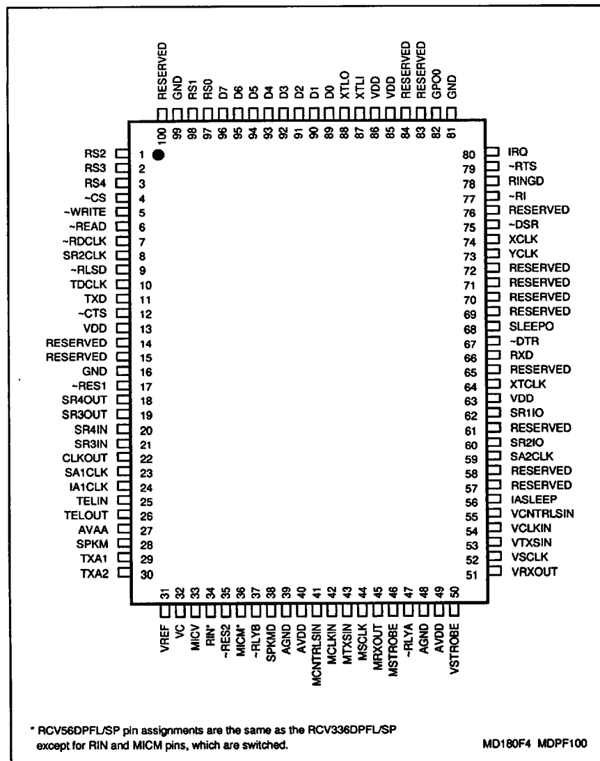
Figure 4. MDP Pin Signals - 100-Pin PQFP
