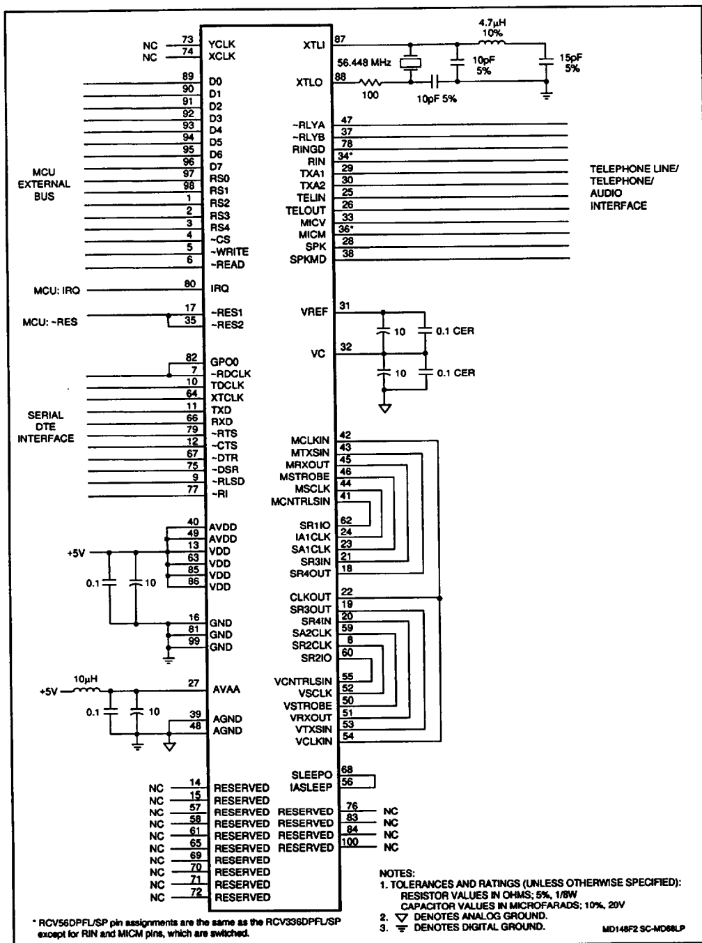
Figure 2. MDP Hardware Interface Signals-100-Pin PQFP
