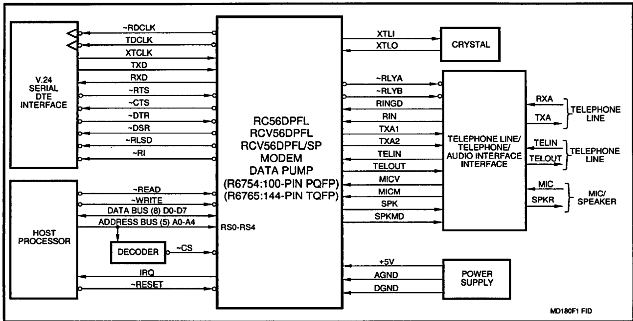
Figure 1. RCV56DPFL/SP MDP Functional Interface
