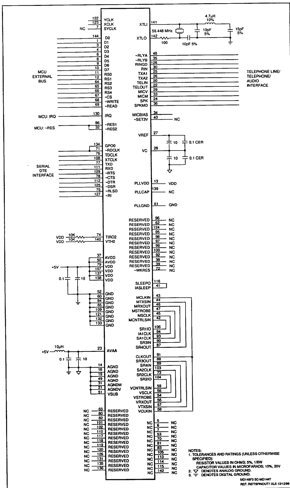
Figure 3. MDP Hardware Interface Signals-144-Pin TQFP
