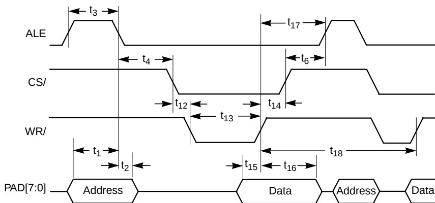
Figure 6.12 Register Write, Multiplexed PAD Bus
