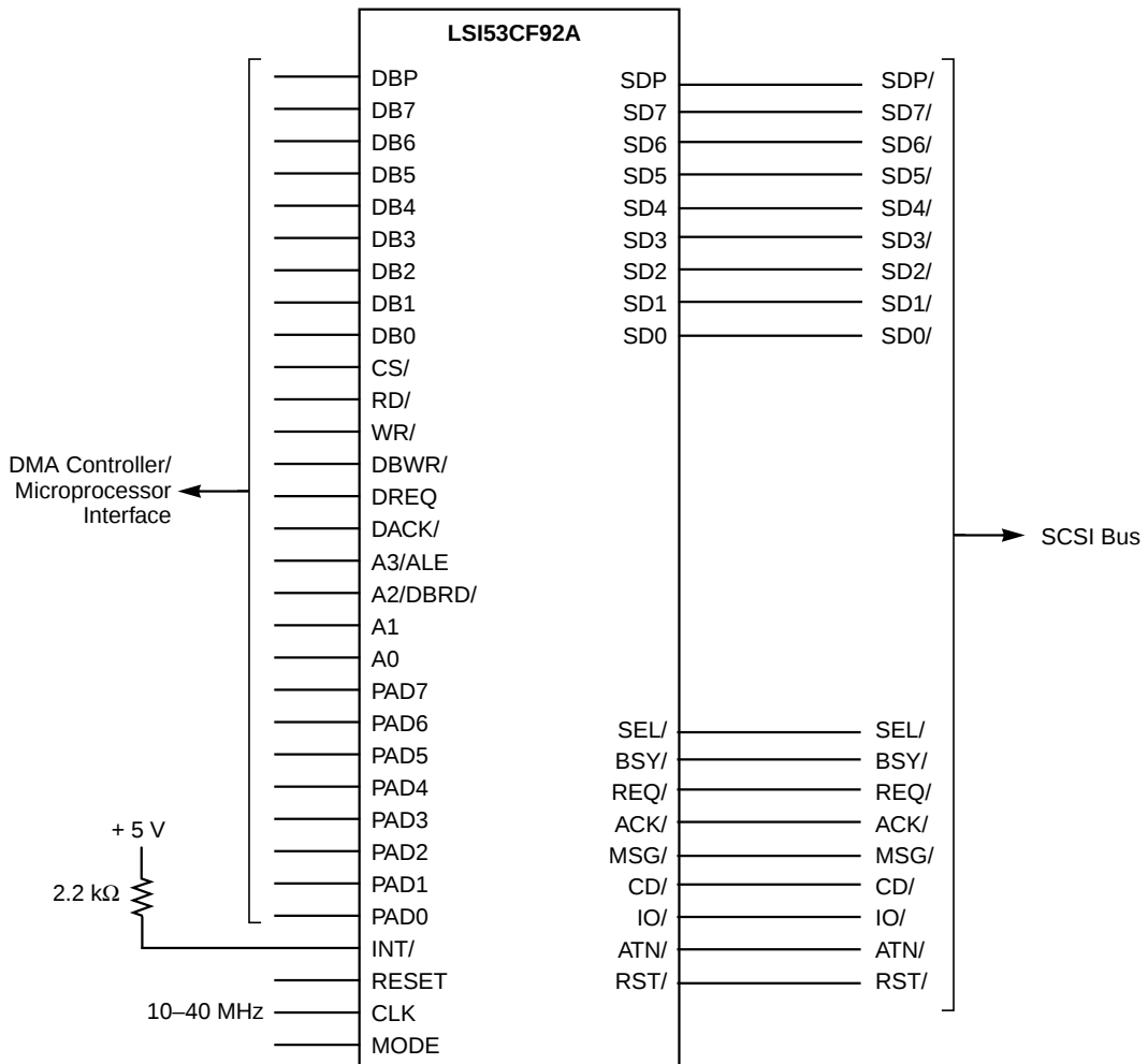
Figure B.1 Single-Pin, SE SCSI Bus Interface Wiring Diagram
