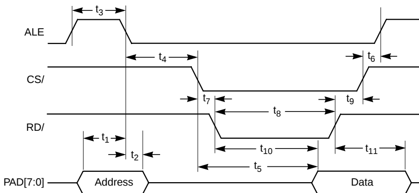
Figure 6.11 Register Read, Multiplexed PAD Bus
