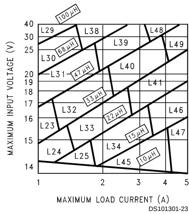
FIGURE 5. LM2677-12
