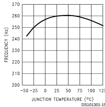
Switching Frequency
