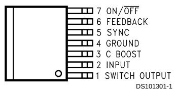
TO-263 Package Top View
