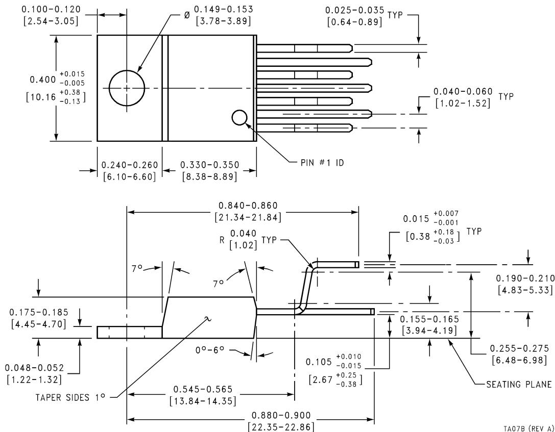
TO-220 Power Package Order Number LM2677T-3.3, LM2677T-5.0, LM2677T-12 or LM2677T-ADJ NS Package Number TA07B
