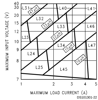
FIGURE 4. LM2677-5.0
