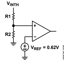
Figure 4. Setting the Adjustable Monitor
