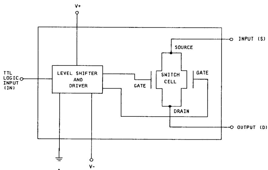
FIGURE 2. Functional diagram.
