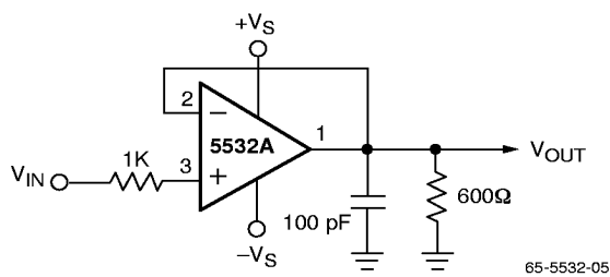
Figure 2. Follower, Transient Response
