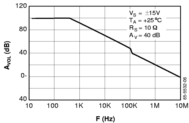
Figure 3. Open Loop Gain vs. Frequency
