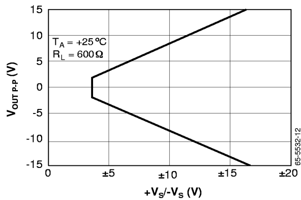
Figure 9. Output Voltage Swing vs. Supply Voltage
