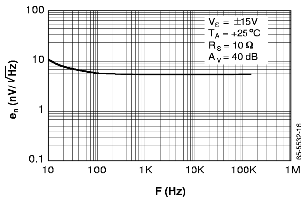
Figure 13. Input Noise Density vs. Frequency
