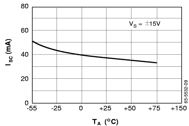
Figure 6. Short Circuit Current vs. Temperature
