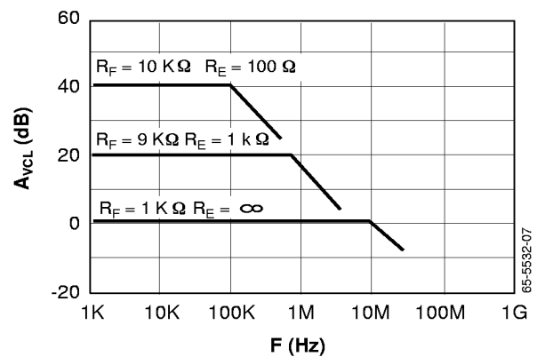
Figure 4. Closed Loop Gain vs. Frequency
