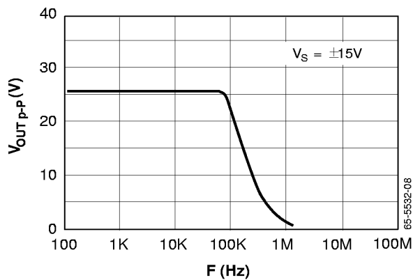
Figure 5. Output Voltage Swing vs. Frequency
