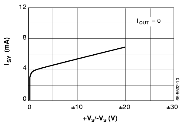
Figure 7. Supply Current vs. Supply Voltage
