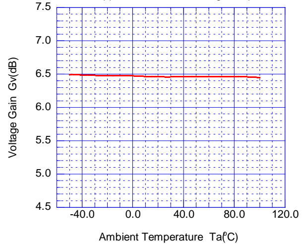
Voltage Gain vs. Temperature 1.0Vpp, 100kHz sinewave signal input
