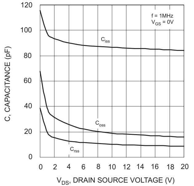
Fig. 12 Capacitance Variation
