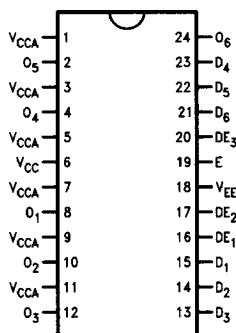
24-Pin DIP
