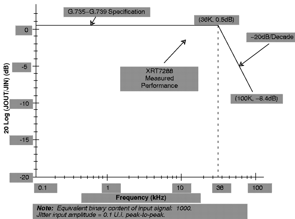
Figure 7. Receive Jitter Transfer Function
