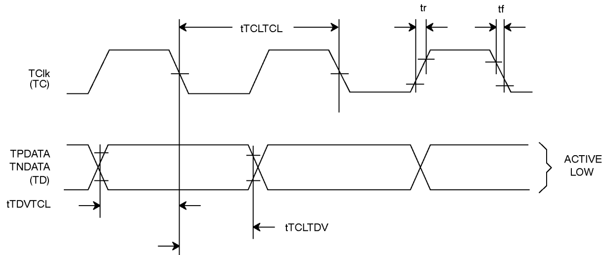
Figure 11. Transmit Timing
