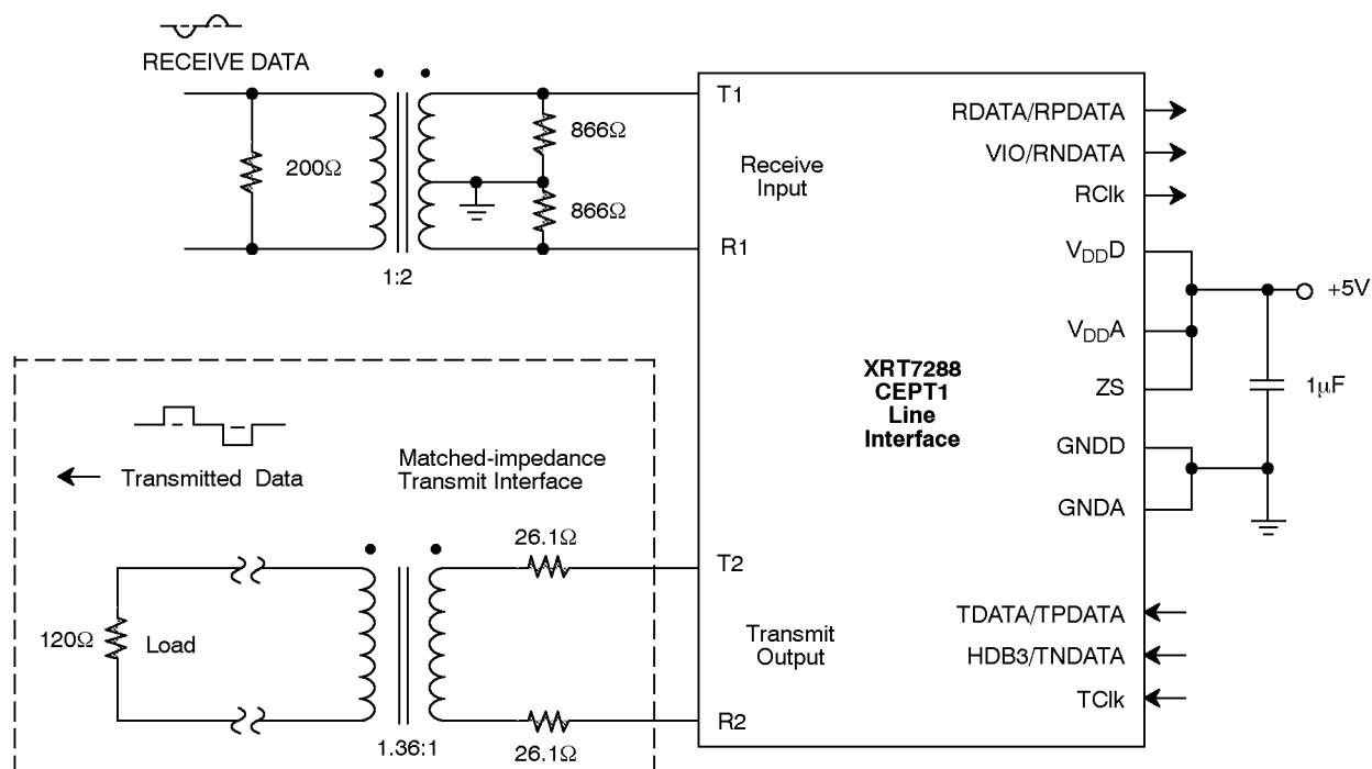
Figure 3. Typical Application Diagram for Shielded Twisted-Pair Environment
