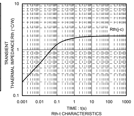
R_{th-t} CHARACTERISTICS
