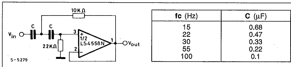
Figure 19 : High-cut Filter (Gv = 0 dB). S G S-THOMSON
