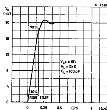
Figure 8 : Transient Response.
