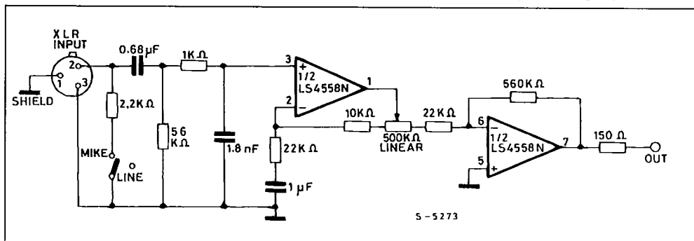
Figure 10 : Mike/Line Preamplifier for Audio Mixers (0 dB to 60 dB continuously variable gain).
