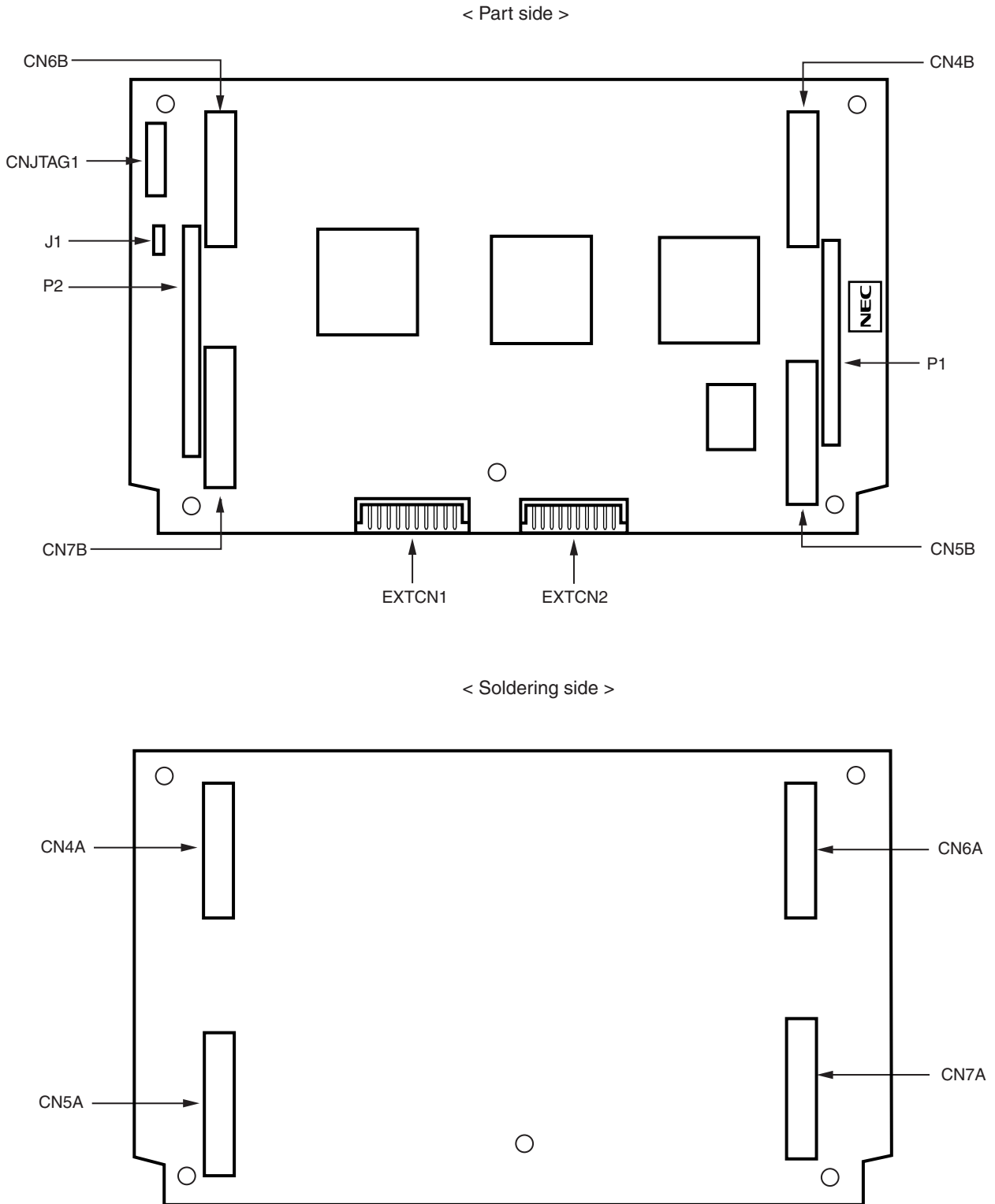
Figure 2-1. Performance Board
