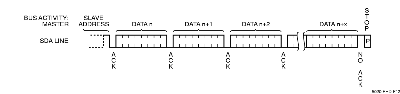
Figure 10. Sequential Read Timing
