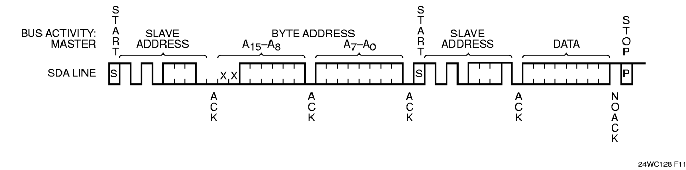
Figure 9. Selective Read Timing
