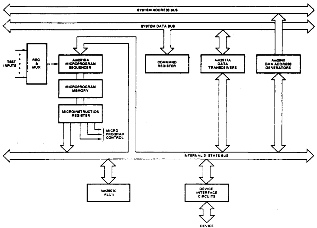
Figure 3. DMA Peripheral Controller Block Diagram.
