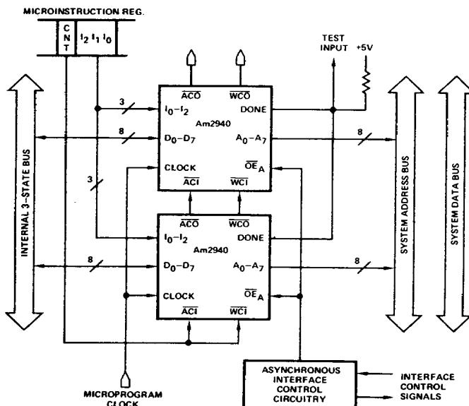
Figure 2. Am2940 Interconnections.
