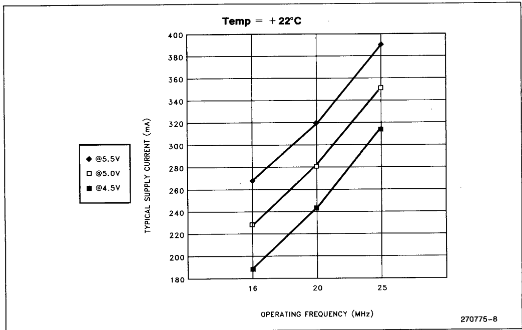
Figure 8. Typical Current vs. Frequency (Room Temp)
