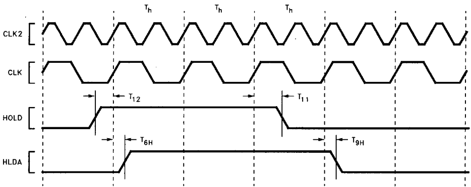
Figure 22. HOLD Timing
