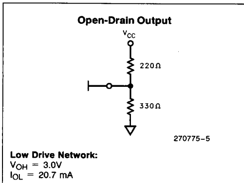
Figure 5. Connection Recommendations for Low Current Drive Network
