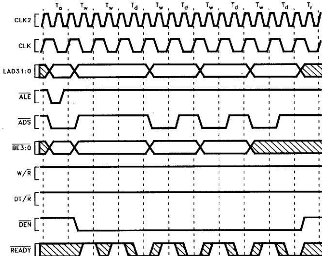
Figure 29. Burst Write Transaction with 2, 1, 1, 1 Wait States
