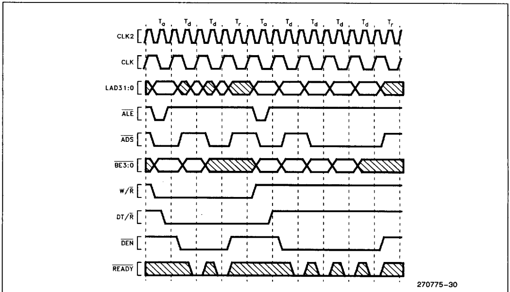
Figure 28. Burst Read and Write Transaction without Wait States
