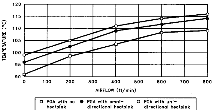
Figure 26. Maximum Allowable Ambient Temperature for the Extended Temperature TA-80960KA 20 MHz in PGA Package
