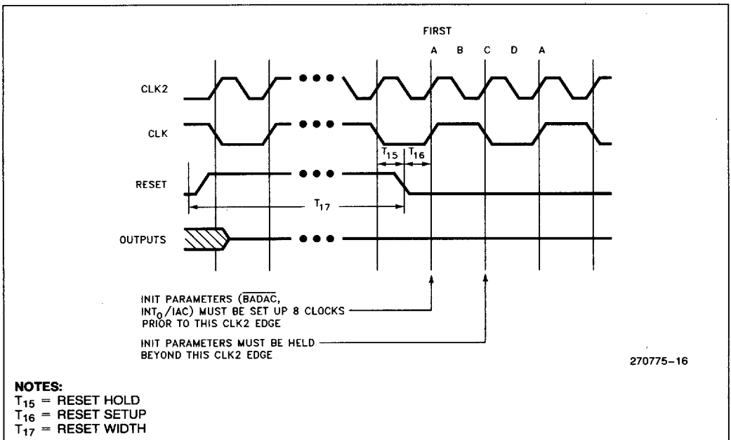
Figure 16. RESET Signal Timing
