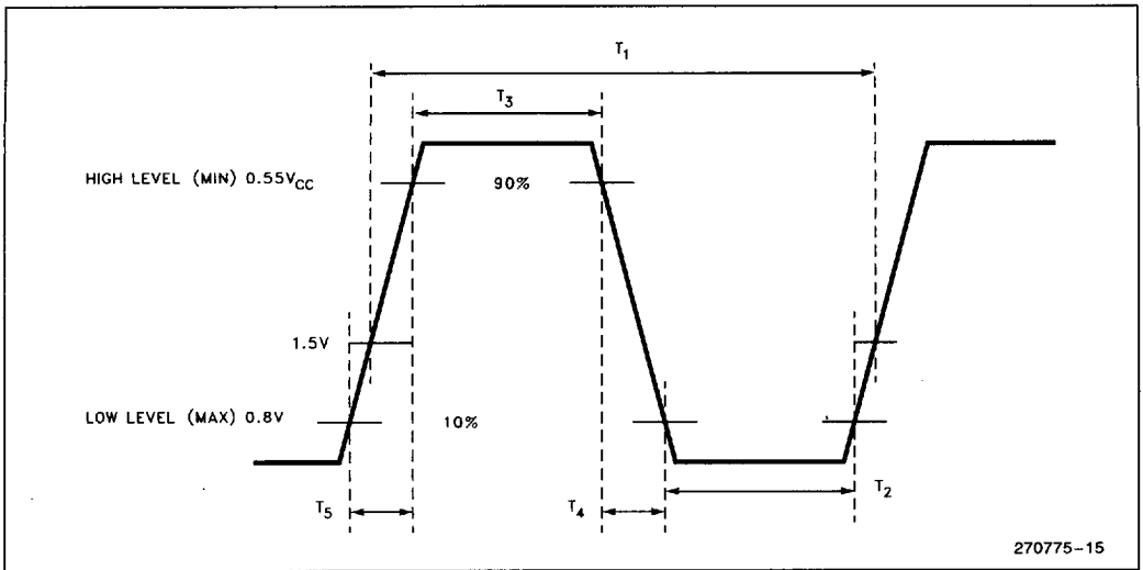
Figure 15. Processor Clock Pulse (CLK2)
