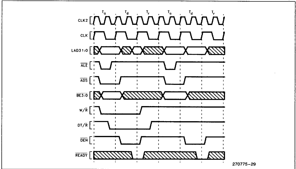
Figure 27. Non-Burst Read and Write Transactions without Wait States
