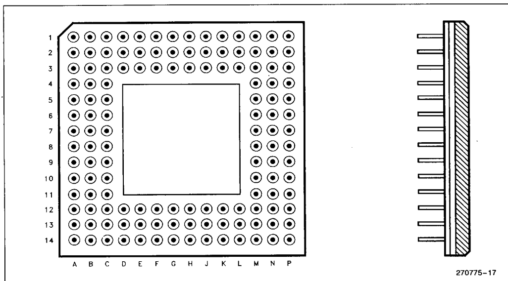
Figure 17. 132-Lead Pin-Grid Array (PGA) Package
