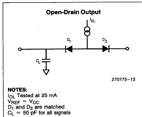
Figure 13. Test Load Circuit for Open-Drain Output Pins
