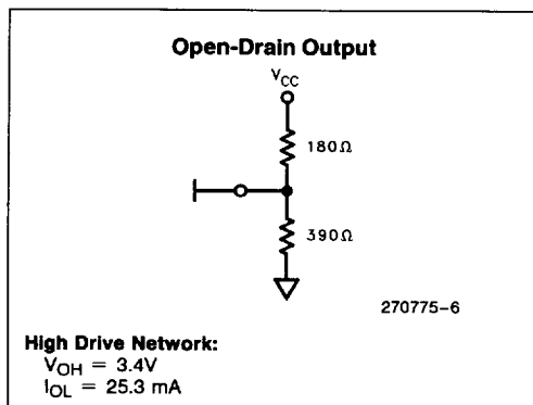
Figure 6. Connection Recommendations for High Current Drive Network
