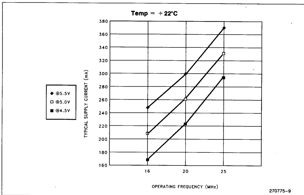
Figure 9. Typical Current vs. Frequency (Hot Temp)
