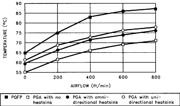
Figure 23. 16 MHz Maximum Allowable Ambient Temperature
