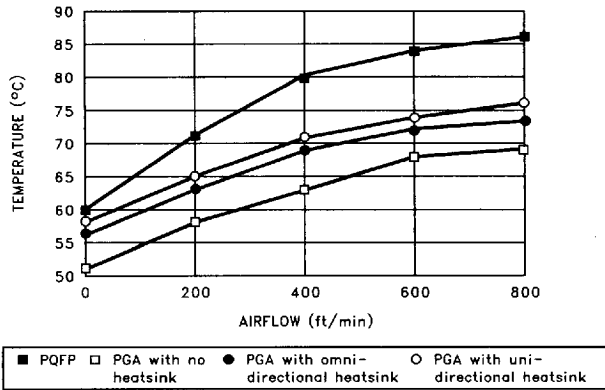
Figure 24. 20 MHz Maximum Allowable Ambient Temperature
