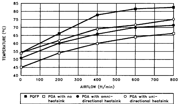
Figure 25. 25 MHz Maximum Allowable Ambient Temperature
