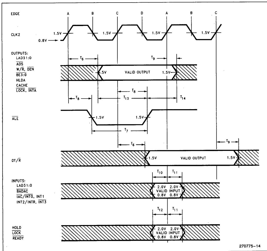
Figure 14. Drive Levels and Timing Relationships for 80960KA Signals
