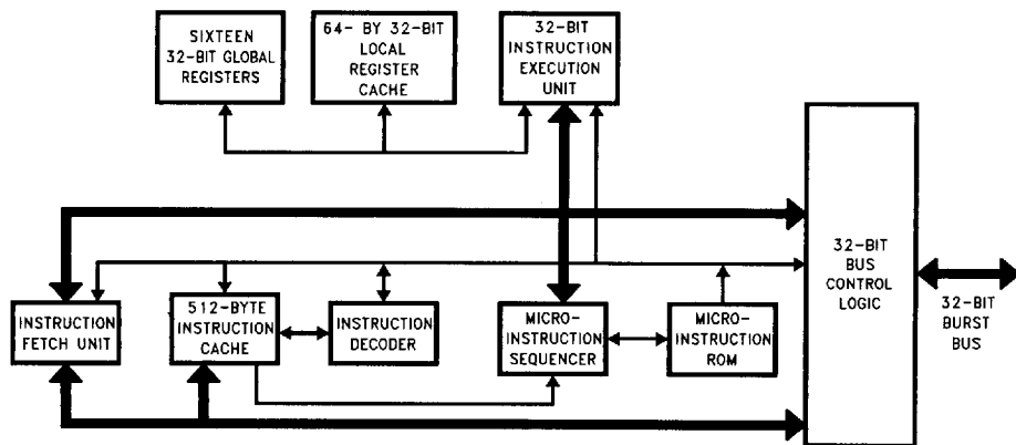
Figure 1. The 80960KA Processor's Highly Parallel Architecture
