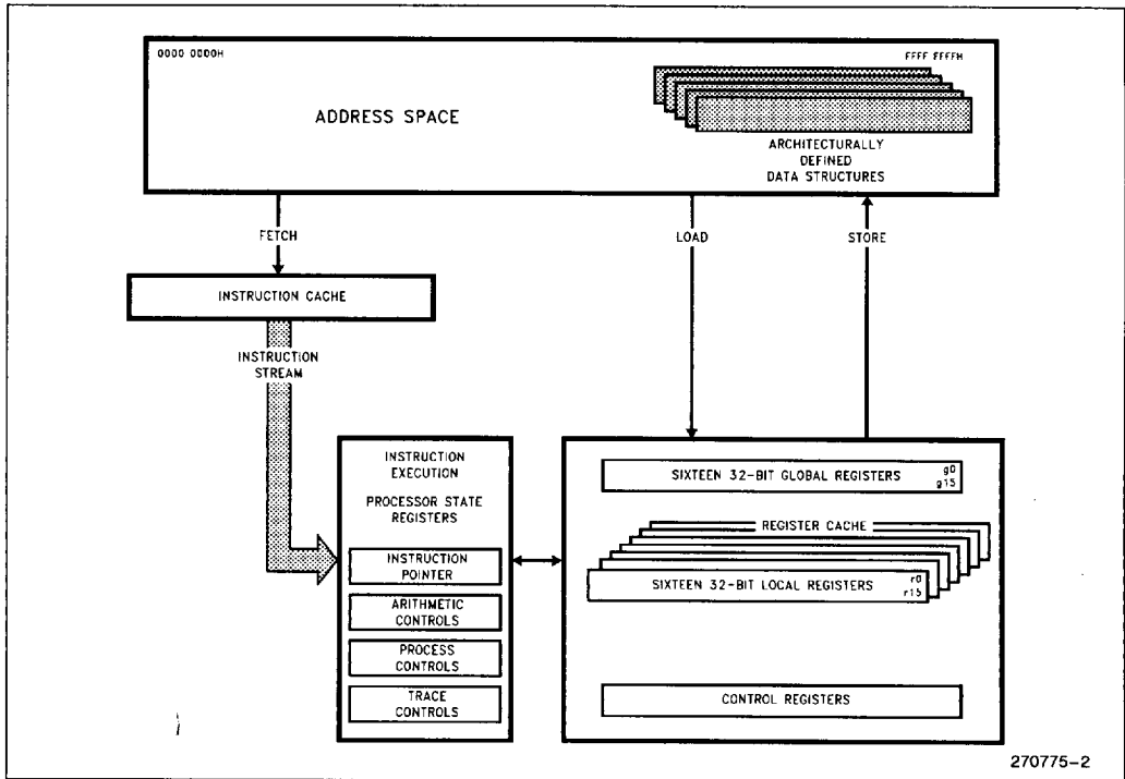
Figure 2. 80960KA Programming Environment
