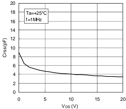
V DS VS. C rss CHARACTERISTICS
