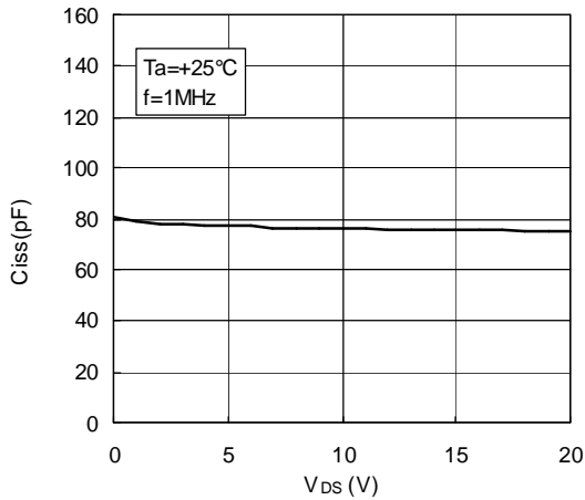
V DS VS. C iss CHARACTERISTICS
