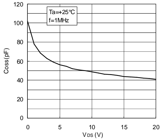
V DS VS. C oss CHARACTERISTICS
