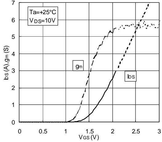
V GS -I DS CHARACTERISTICS
