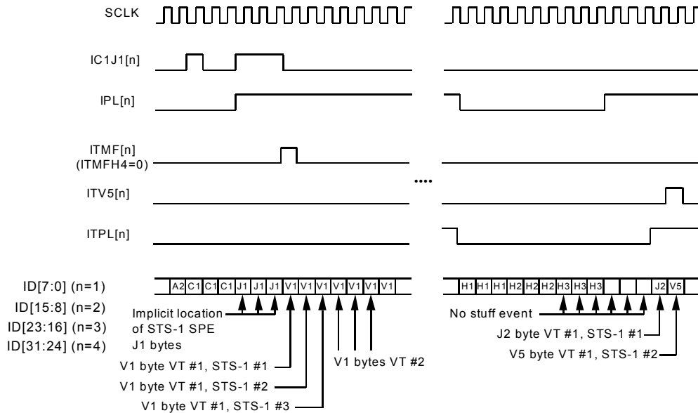
Figure 20 - STM-1 Input Bus Timing - STS-1 / AU3 (VT/TU Pointer Interpretation Disabled)
