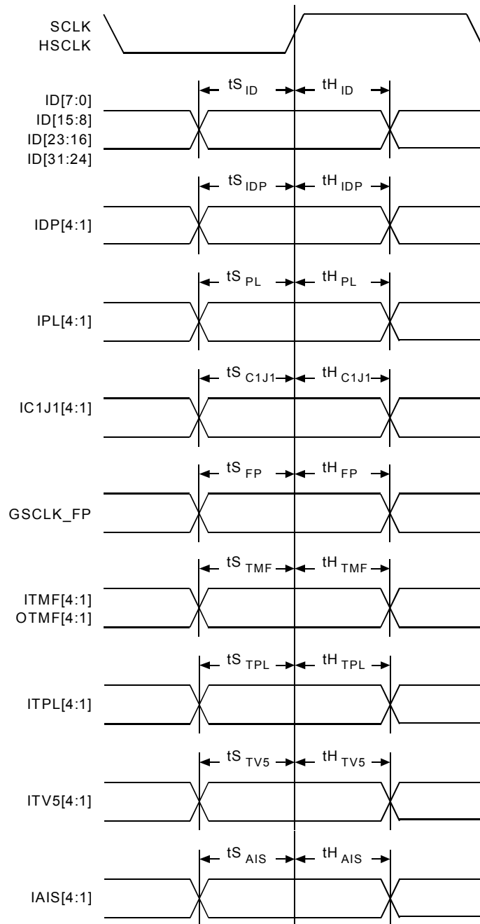
Figure 34 - Input Timing
