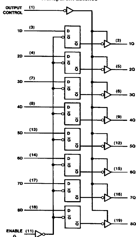
Transparent Latches
