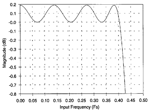
Figure 15. DAC Passband Ripple.
