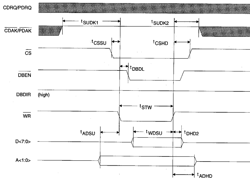
I/O Write Cycle
