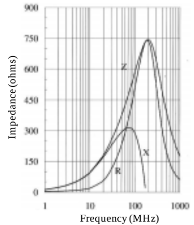
BMB-2B-0600M4-N2
