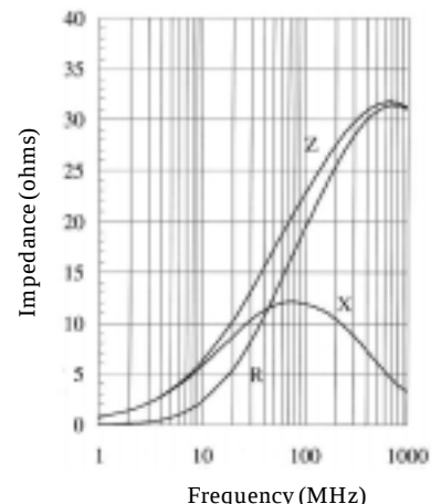
BMB-2A-0020P-N1
