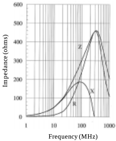
BMB-2B-0300M4-N2
