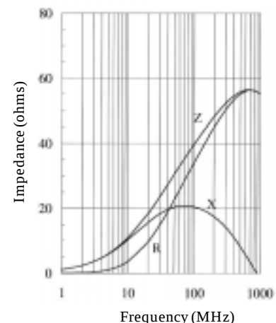
BMB-2A-0040P-N1
