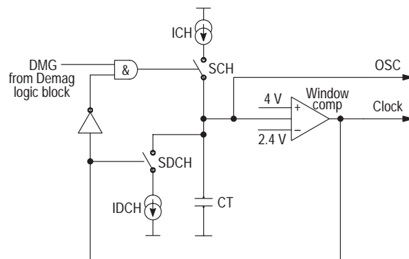
Figure 4. Oscillator Block
