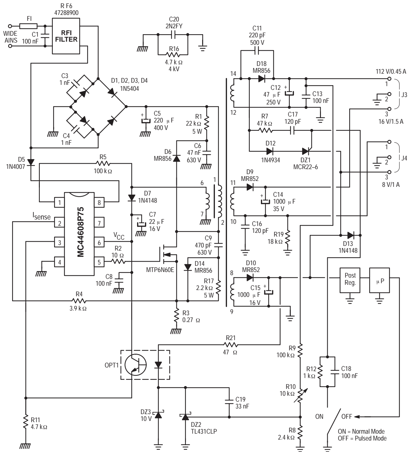
Figure 17. Typical Application
