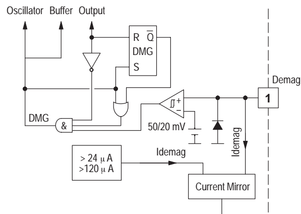
Figure 3. Demagnetization Block
