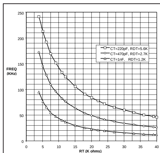
Figure 9: fosc versus effective RT (tDEAD = 1.0 usec)
