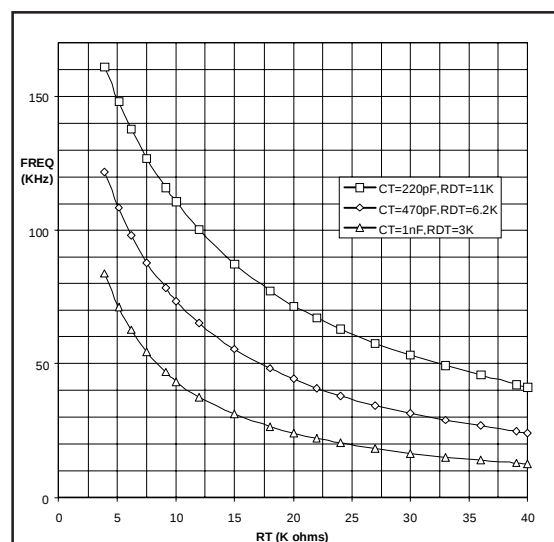
Figure 8: fosc versus effective RT (tDEAD = 2.0 usec)
