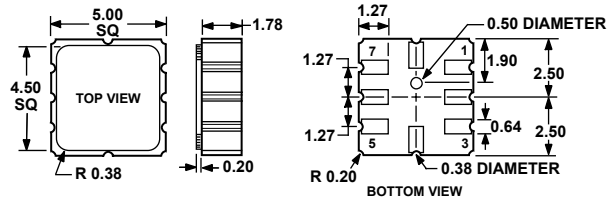
Figure 23. 8-Terminal Ceramic Leadless Chip Carrier [LCC] (E-8)
