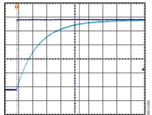
Figure 21. Turn-On Time— C_x, C_y = 0.1 \mu F , Time Scale = 2 ms/DIV
