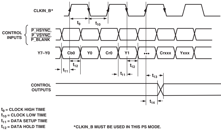
Figure 4. PS 4:2:2 8-Bit Interleaved at 27 MHz \overline{HS\_SYNC}/\overline{VS\_SYNC} Input Mode [Input Mode 100]
