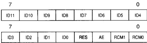
Figure 17. Identifier mapping in the Identifier buffer
