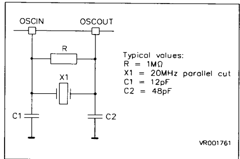
Figure 21. ST9560 Oscillator
