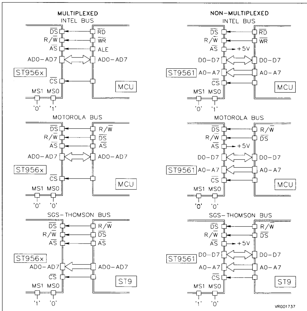
Figure 15. Micro Interface Schematics
