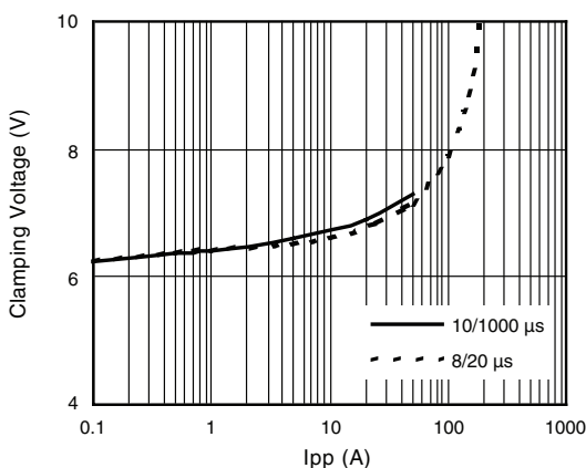
Figure 4. Clamping Voltage vs. Peak Pulse Current ( T_J initial = 25\text{ }^\circ\text{C} )
