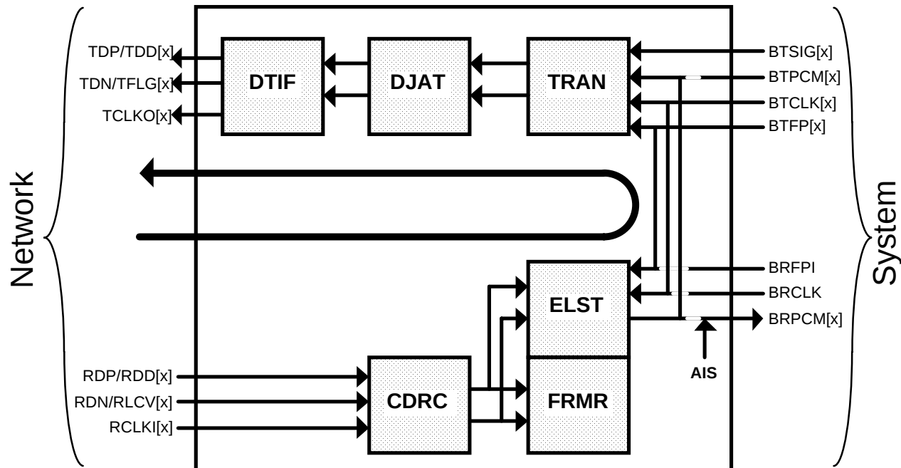
Figure 28 - Payload Loopback
