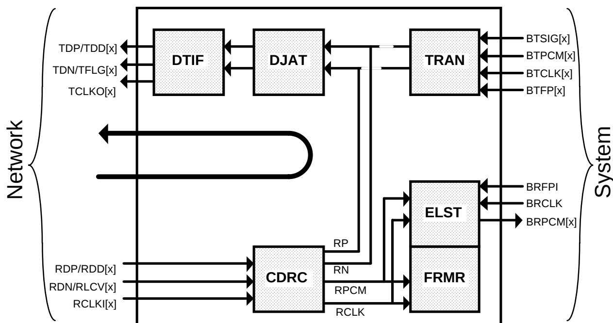
Figure 29 - Line Loopback
