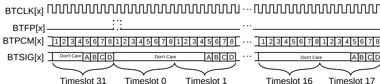
Figure 18 - Transmit Backplane Interface
